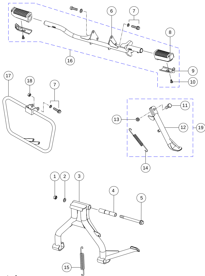
CENTER STAND &amp; FOOTREST ASSY.
