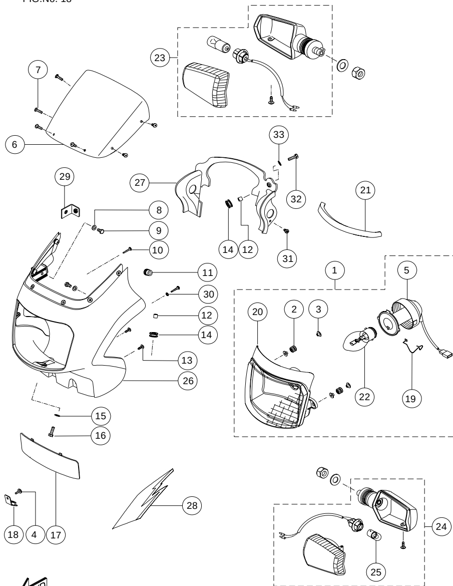
HEAD LAMP ASSEMBLY &amp; TSL LH, RH
