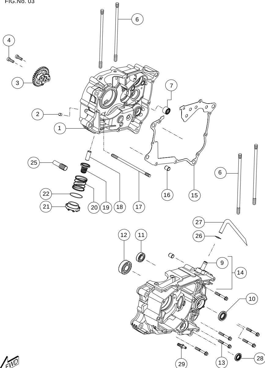
CRANKCASE LH, RH &amp; OIL PUMP ASSY.
