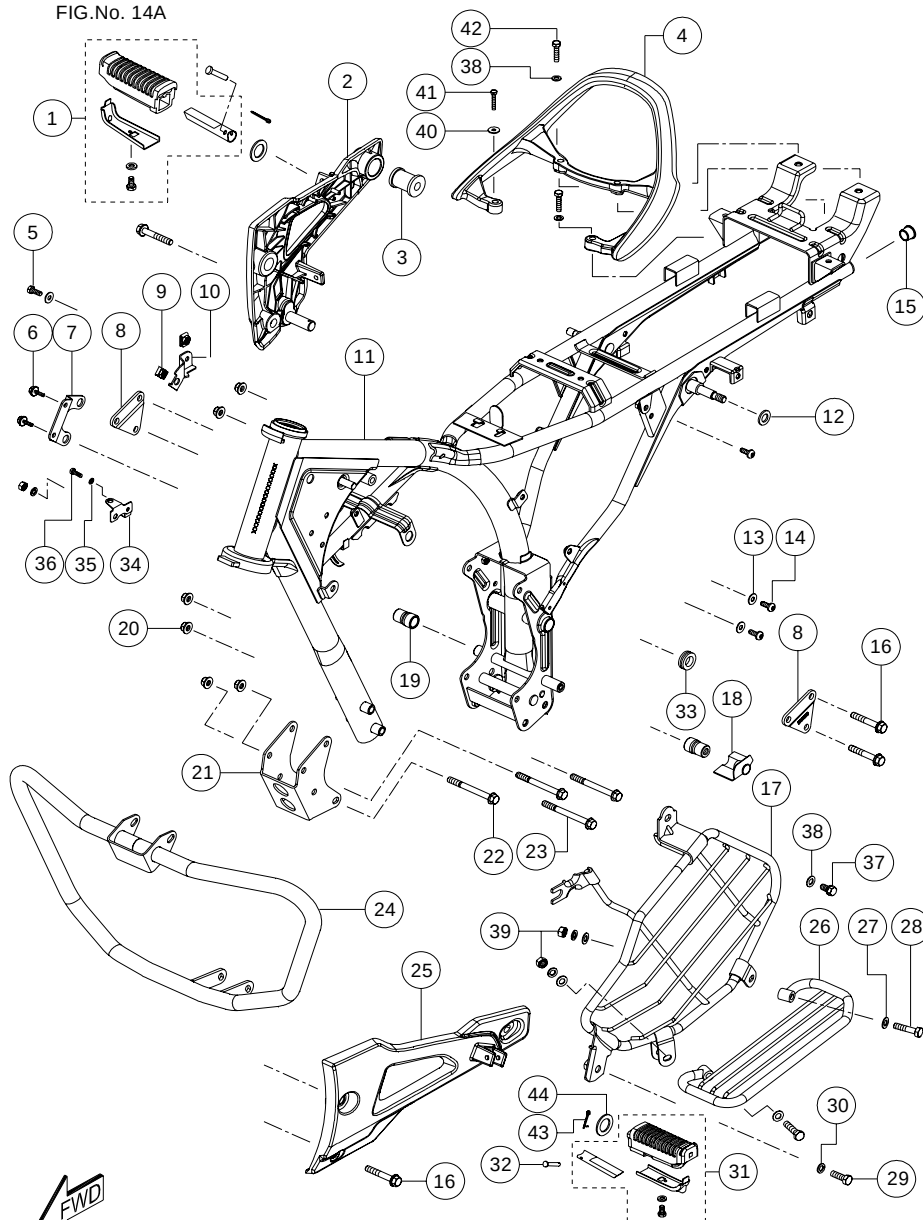
FRAME &amp; SAREE GUARD ASSEMBLY(GLX)
