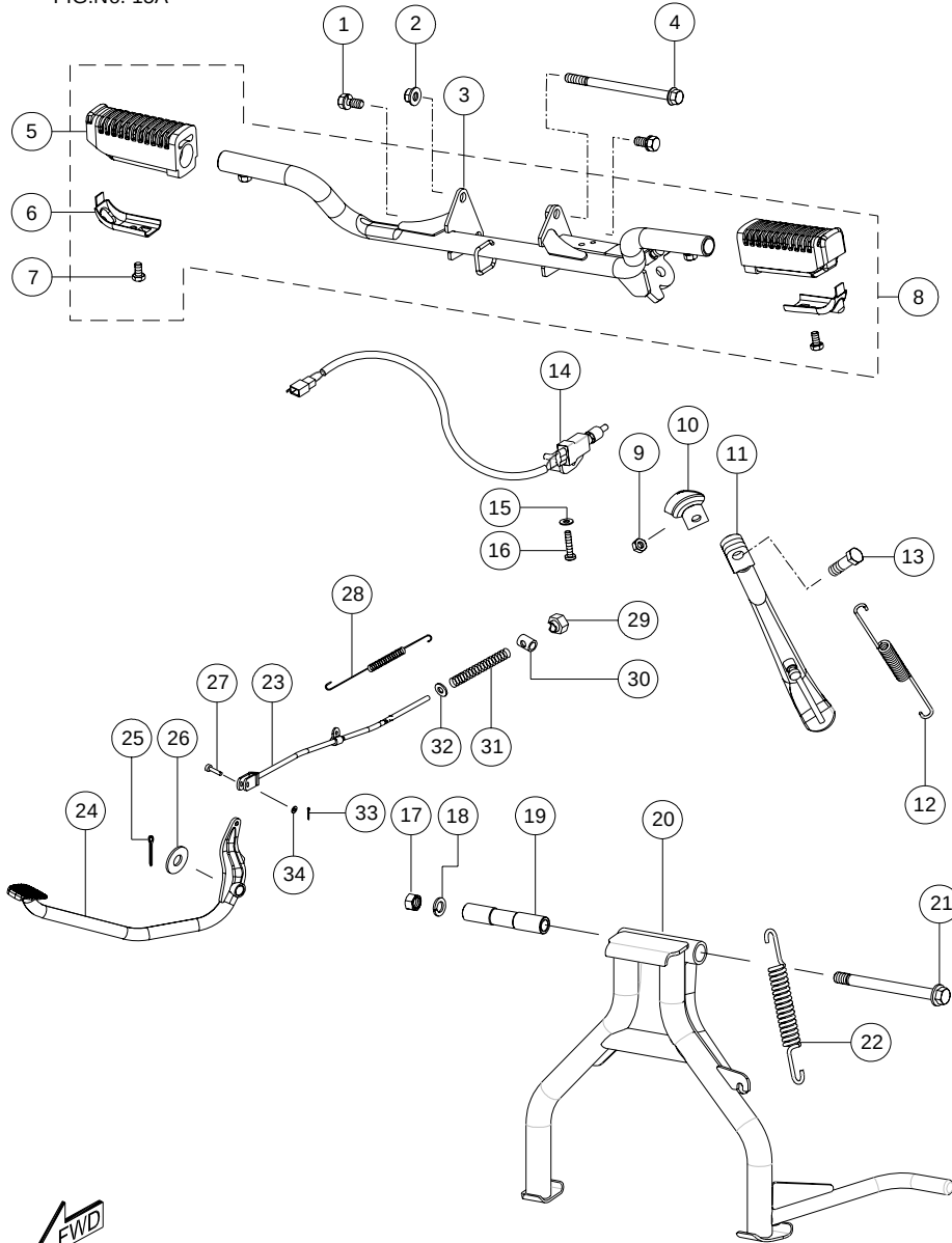
CENTER STAND & FOOTREST ASSY. (GLX)
