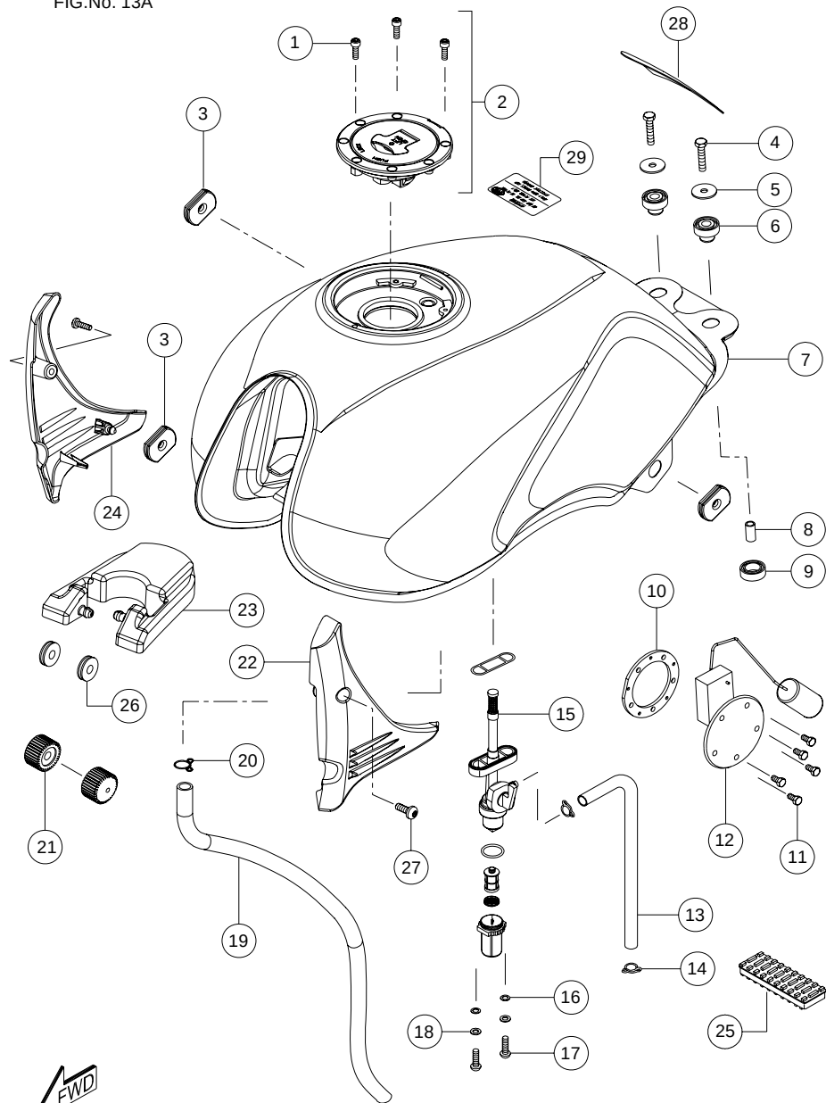
FUEL TANK &amp; FUEL COCK ASSY. (GLX)
