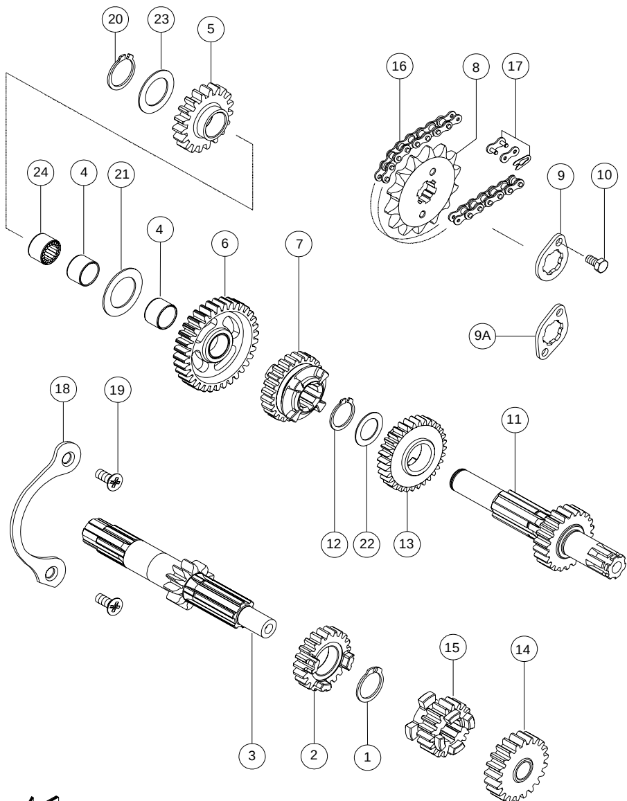
TRANSMISSION ASSEMBLY
