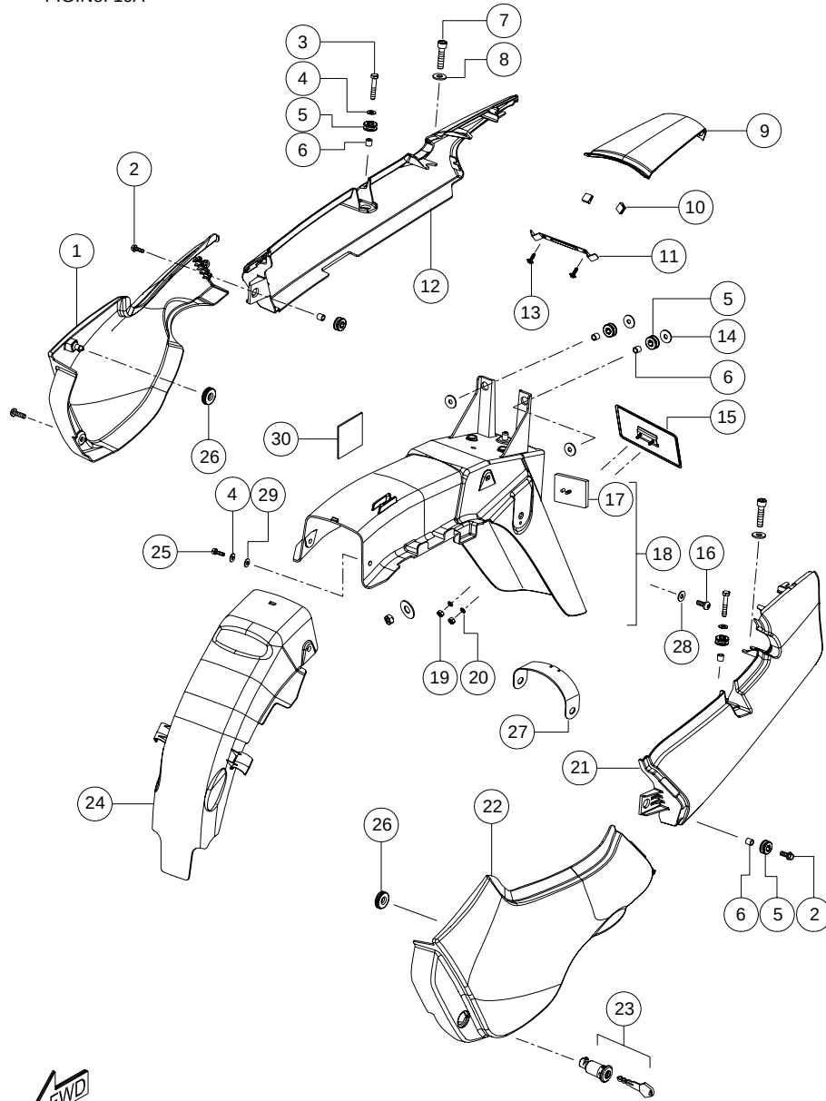
PANEL L,R &amp; REAR FENDER ASSY. (GLX)
