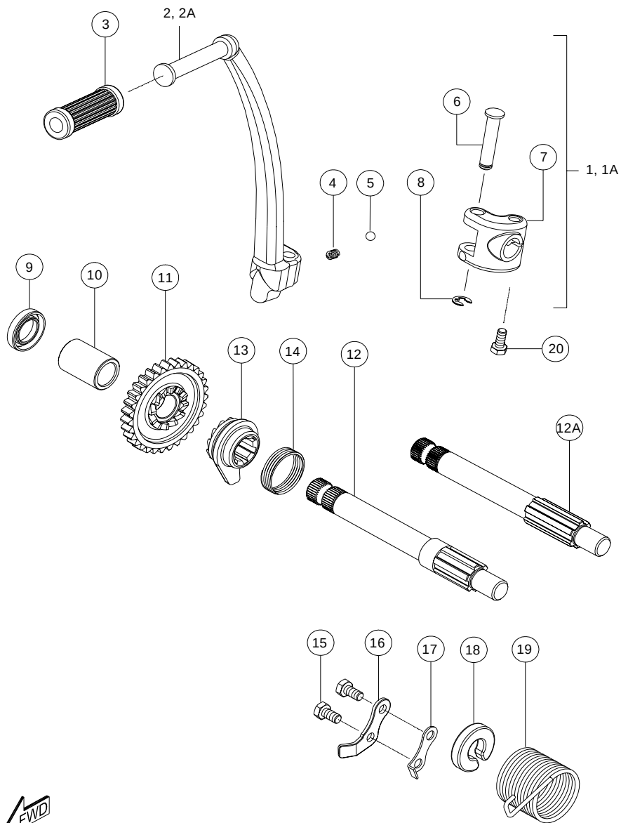
KICK STARTER ASSEMBLY
