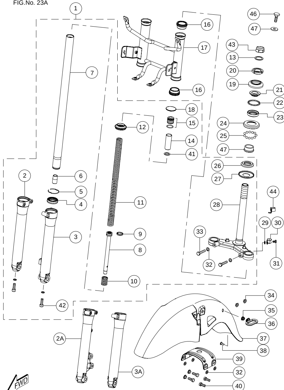
FRONT FORK ASSEMBLY (GLX)
