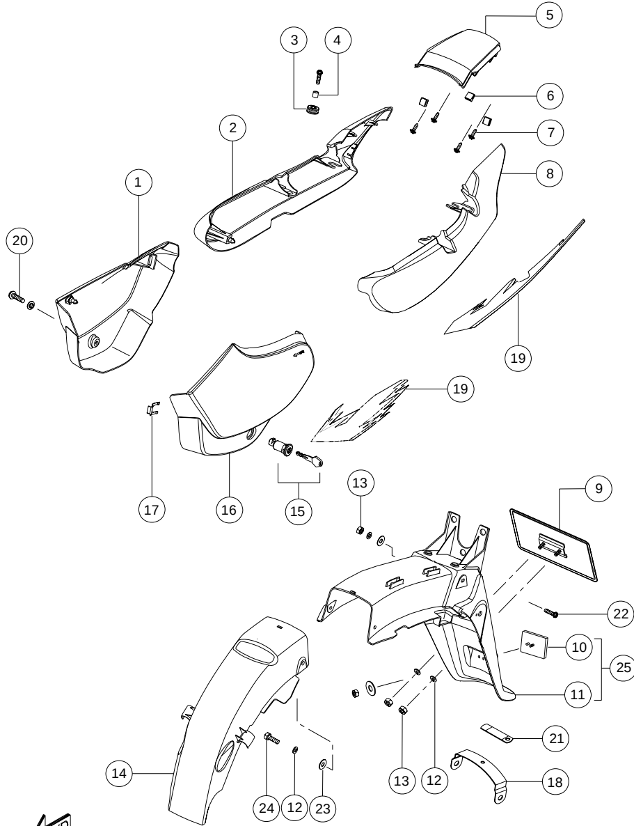
PANEL L,R &amp; REAR FENDER ASSY.
