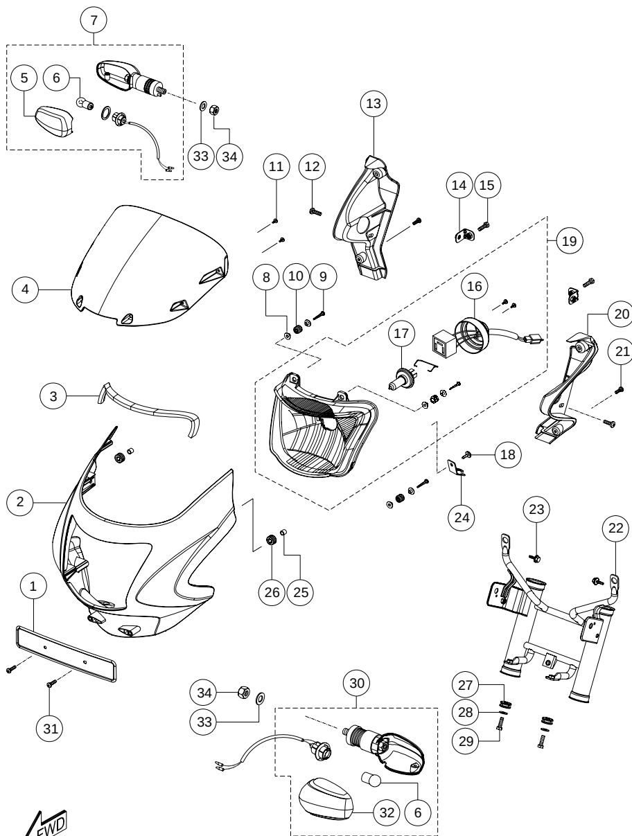
HEAD LAMP ASSEMBLY &amp; TSL LH,RH (GLX)
