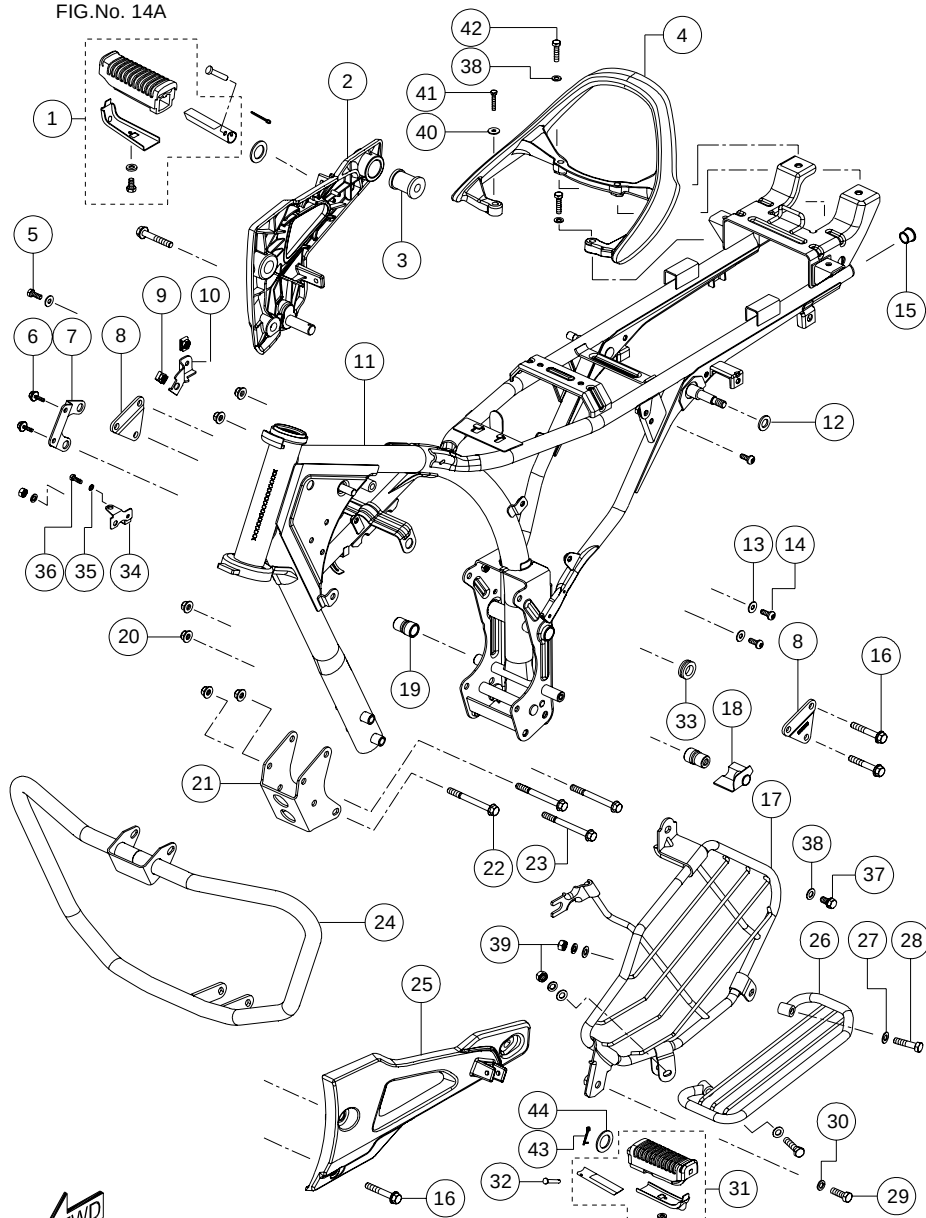
FRAME & SAREE GUARD ASSEMBLY(GLX)
