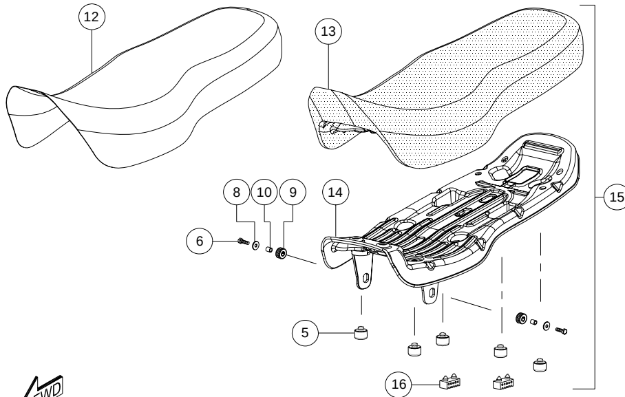
SEAT ASSEMBLY
