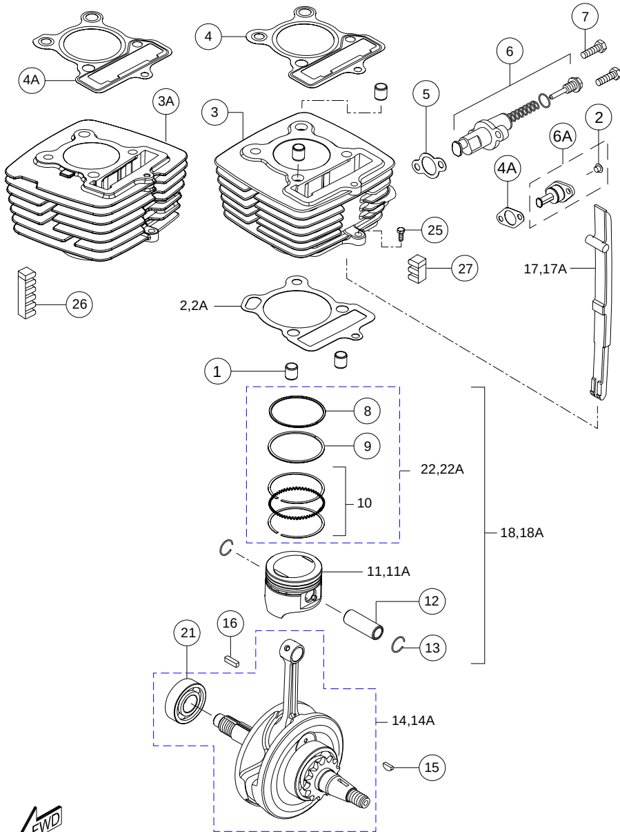
CYLINDER BLOCK &amp; CRANK SHAFT ASSY.
