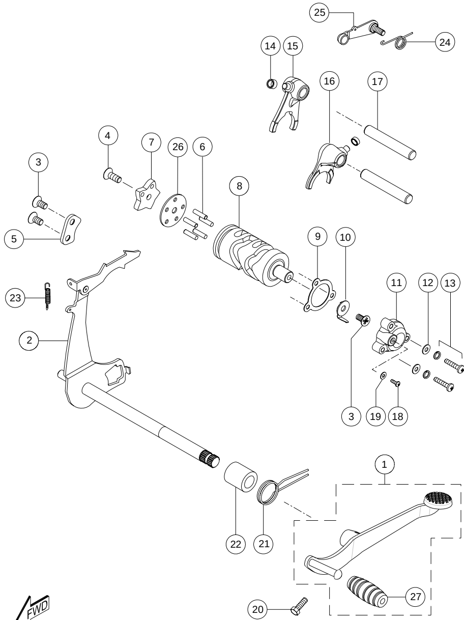
GEAR SHIFT MECHANISM ASSY.
