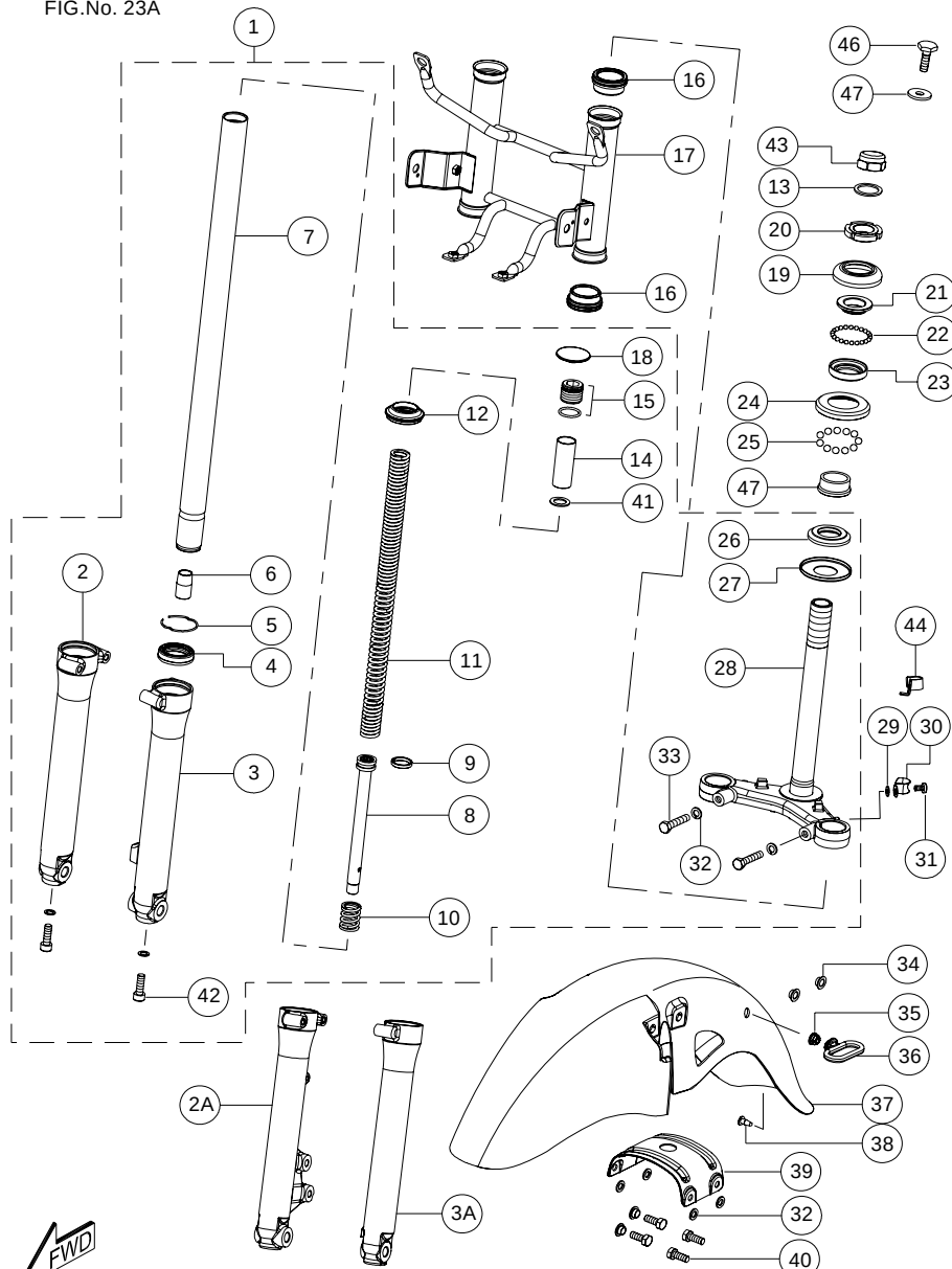
FRONT FORK ASSEMBLY (GLX)
