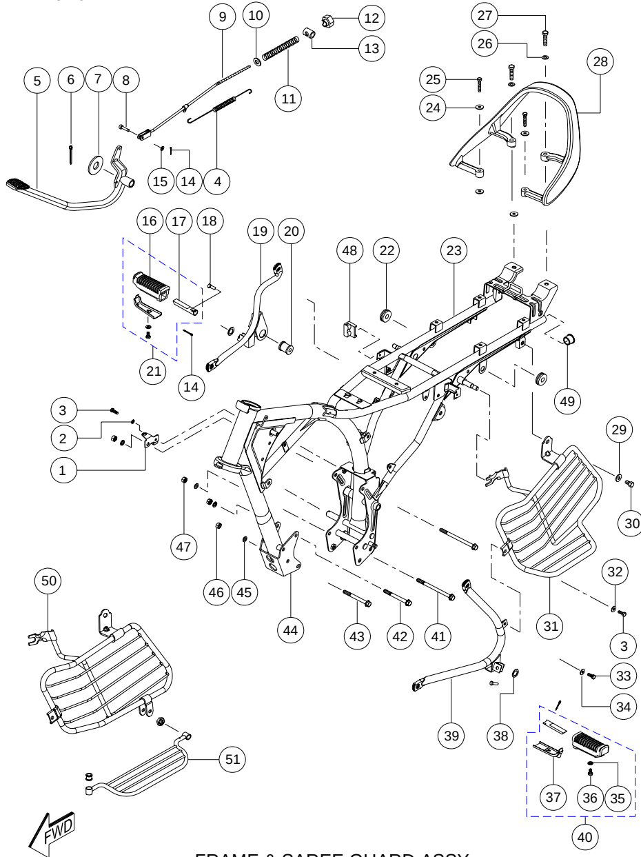
FRAME &amp; SAREE GUARD ASSY.
