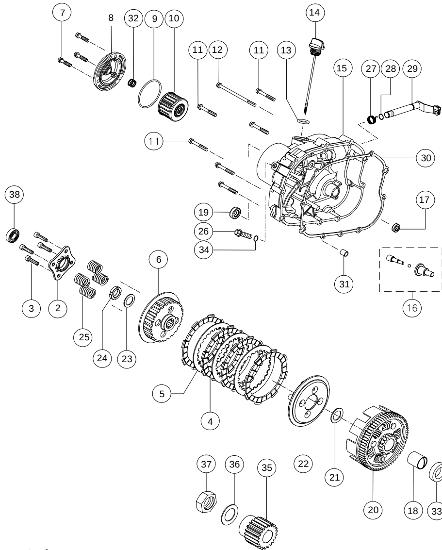
CLUTCH &amp; COVER CLUTCH ASSY.
