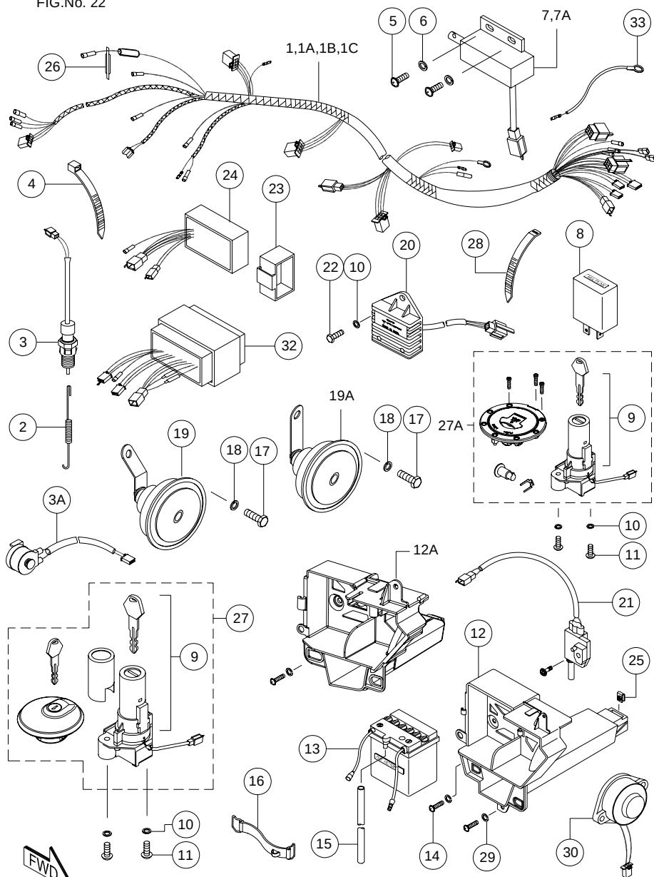
WIRING HARNESS, CDI UNIT &amp; BATTERY ASSY.
