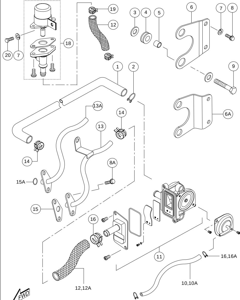
SECONDARY AIR INJECTION ASSY.
