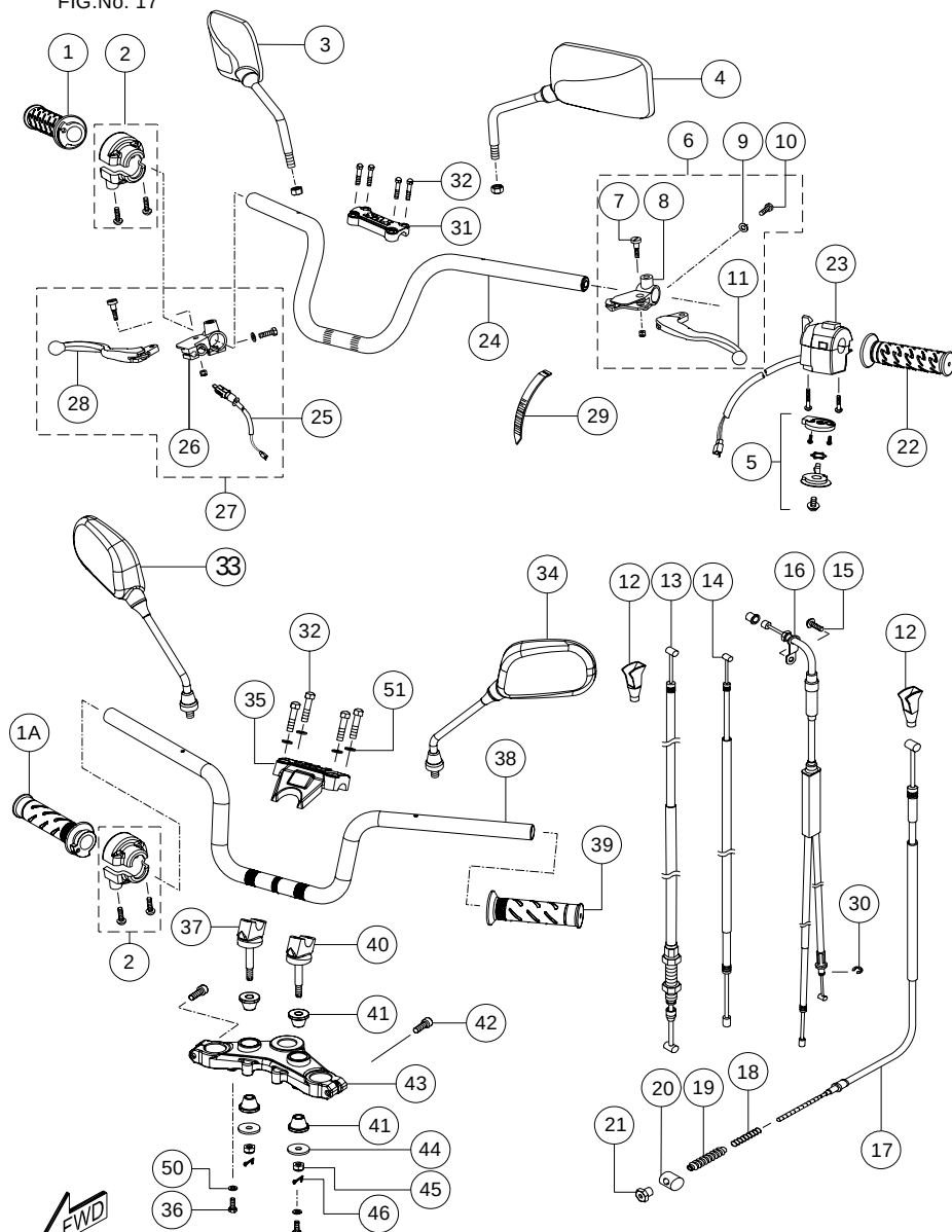
HANDLE BAR SWITCH & CABLE ASSY.
