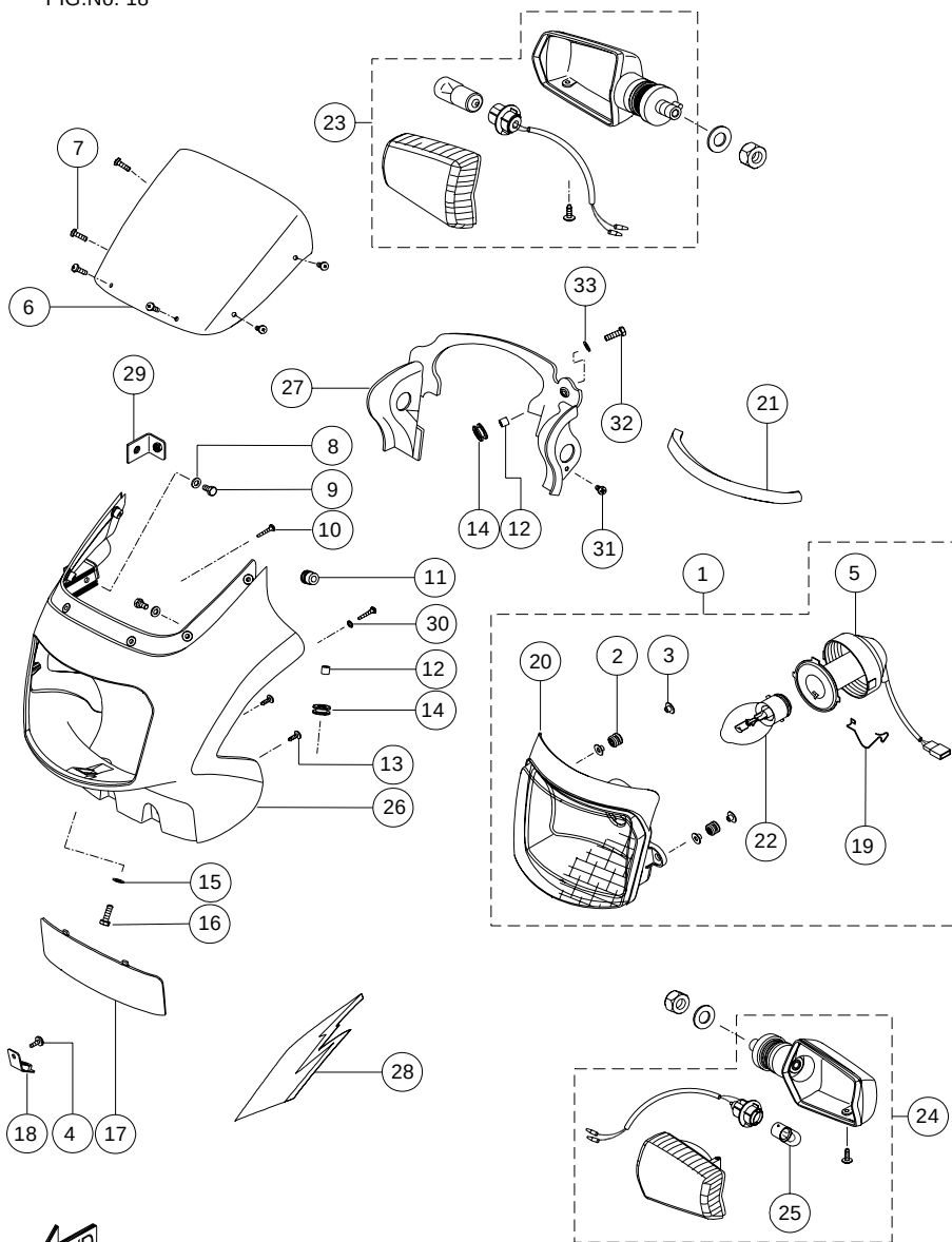
HEAD LAMP ASSEMBLY &amp; TSL LH, RH
