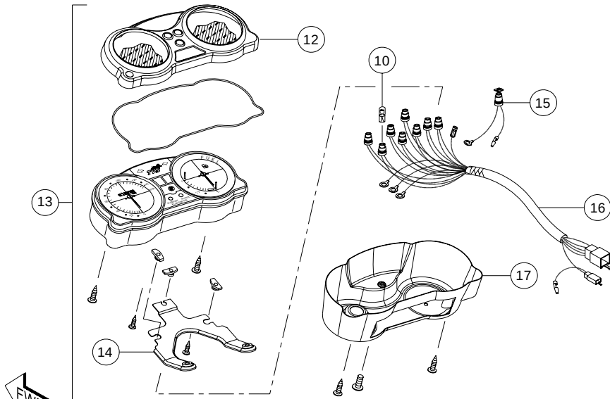
SPEEDOMETER ASSEMBLY
