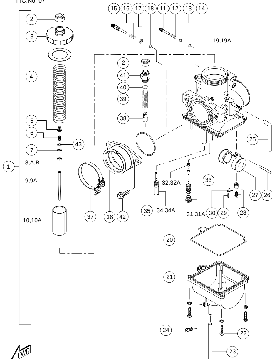
CARBURETTOR ASSEMBLY
