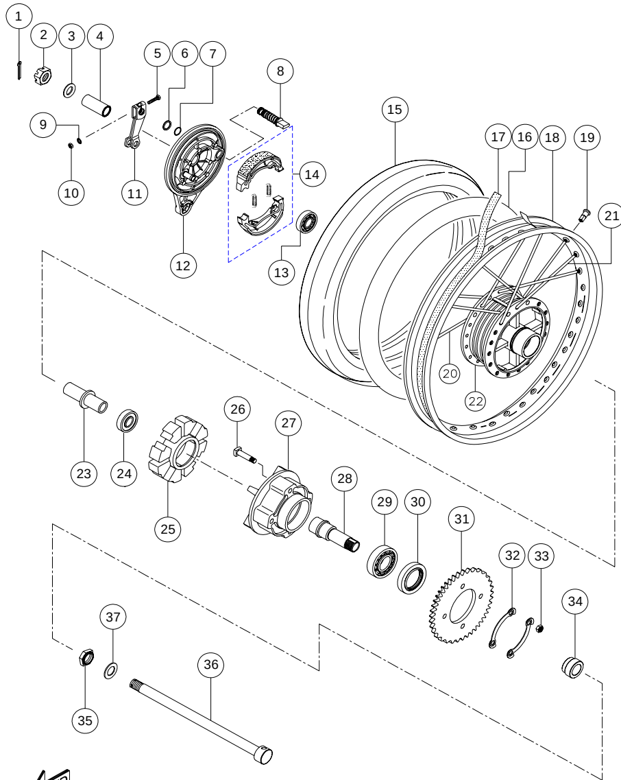
REAR WHEEL ASSEMBLY (GLX)
