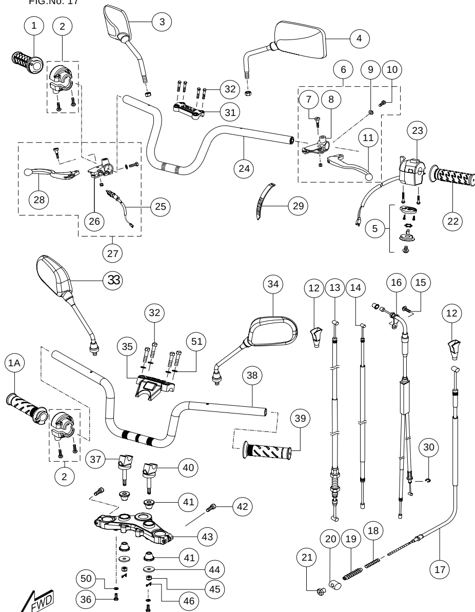
HANDLE BAR SWITCH &amp; CABLE ASSY.
