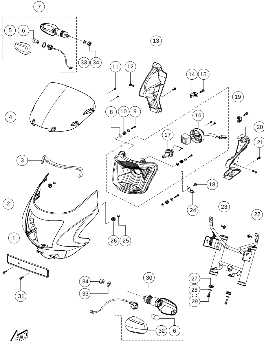
HEAD LAMP ASSEMBLY &amp; TSL LH,RH (GLX)
