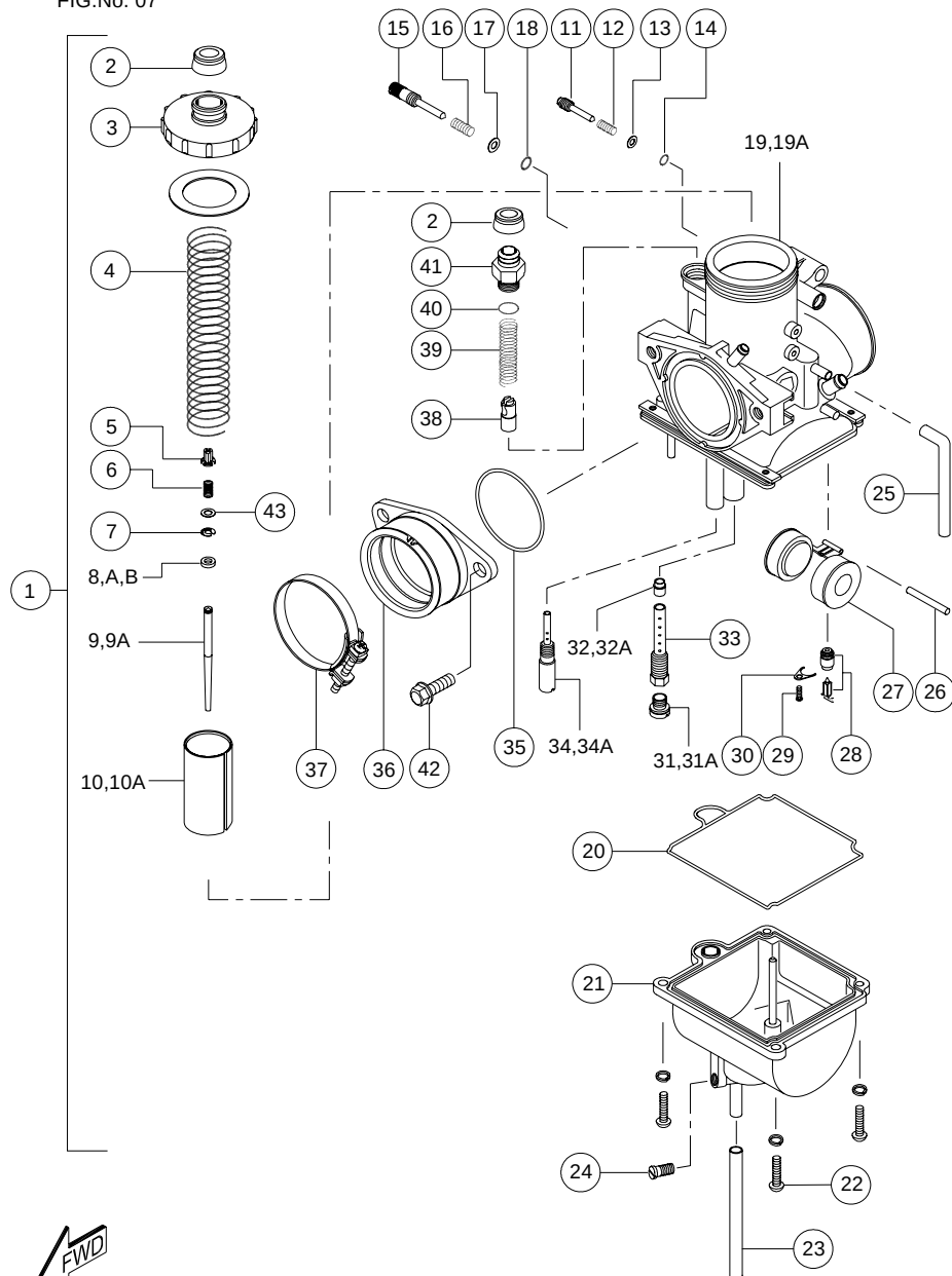
CARBURETTOR ASSEMBLY
