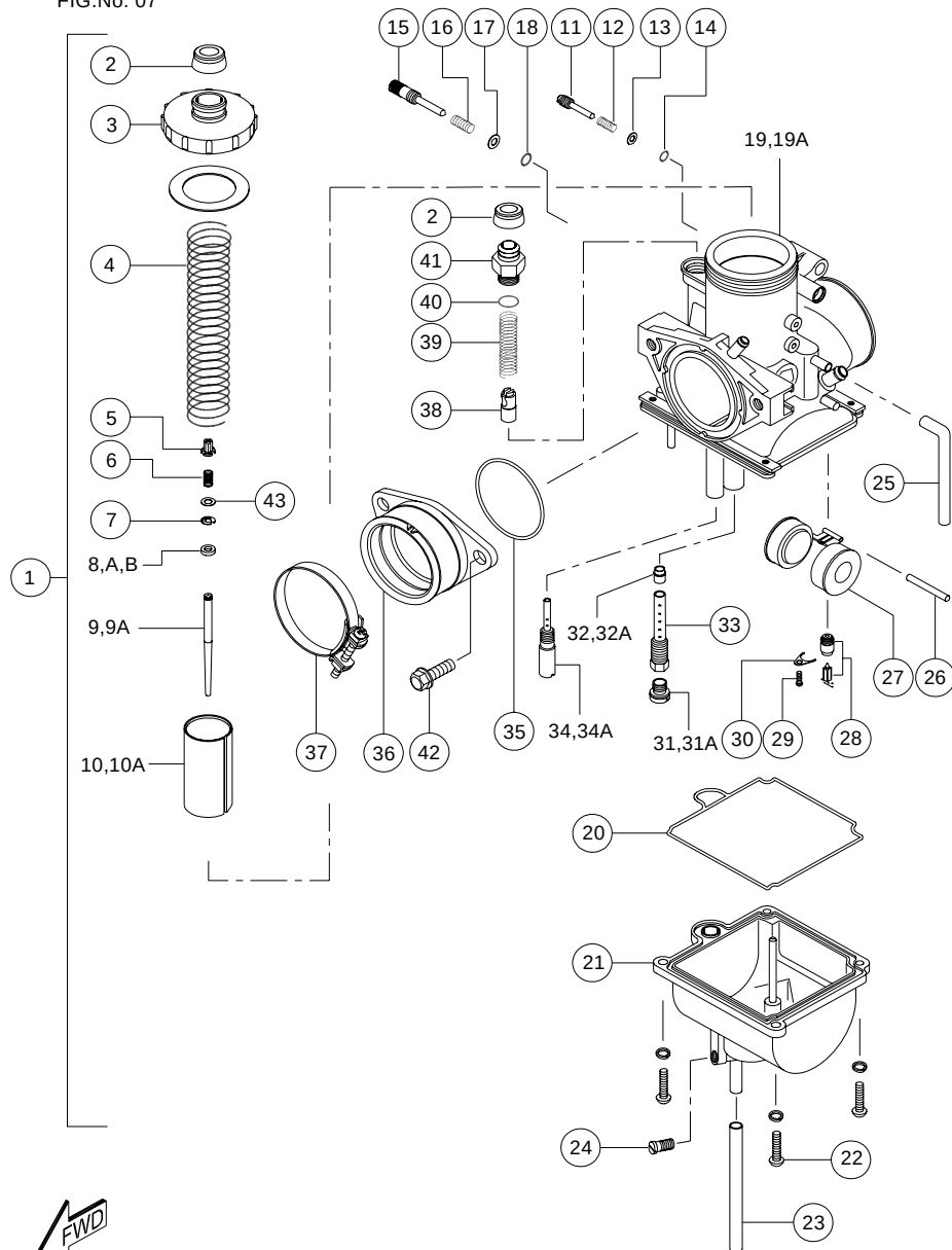
CARBURETTOR ASSEMBLY
