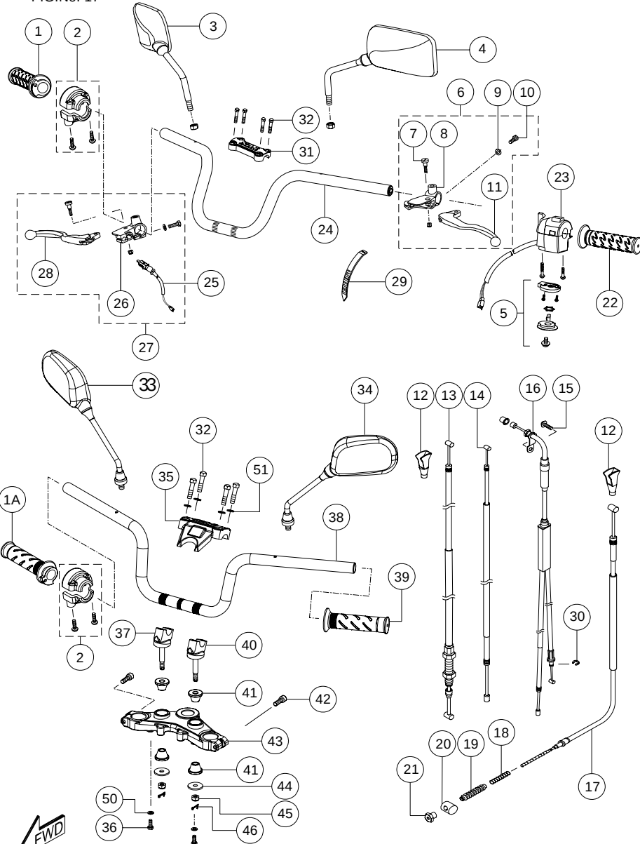
HANDLE BAR SWITCH &amp; CABLE ASSY.
