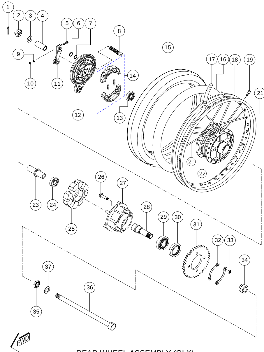
REAR WHEEL ASSEMBLY (GLX)
