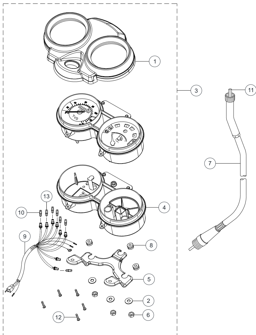
SPEEDOMETER ASSEMBLY
