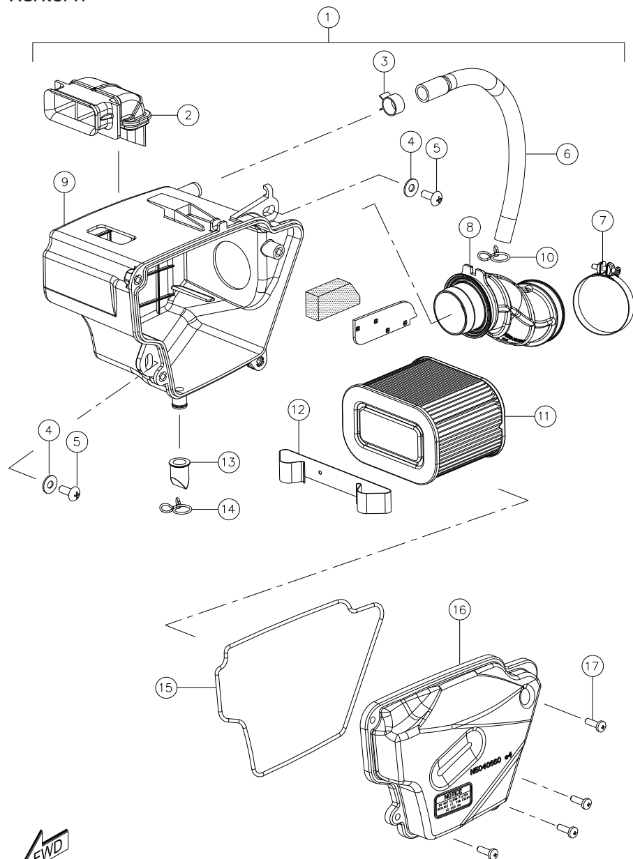
AIR CLEANER ASSEMBLY
