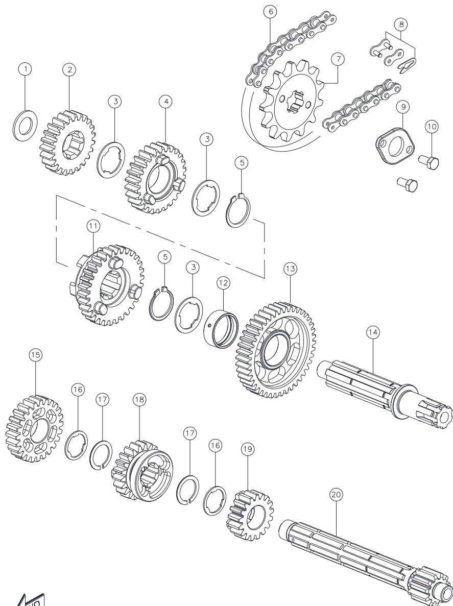
TRANSMISSION ASSEMBLY
