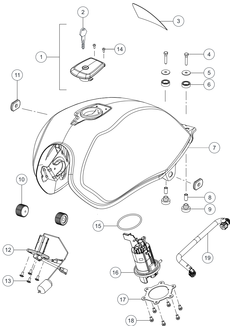
FUEL TANK ASSEMBLY
