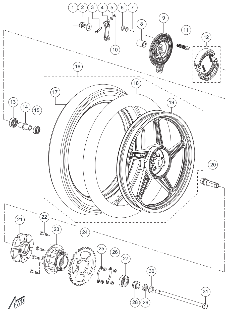
REAR WHEEL ASSEMBLY
