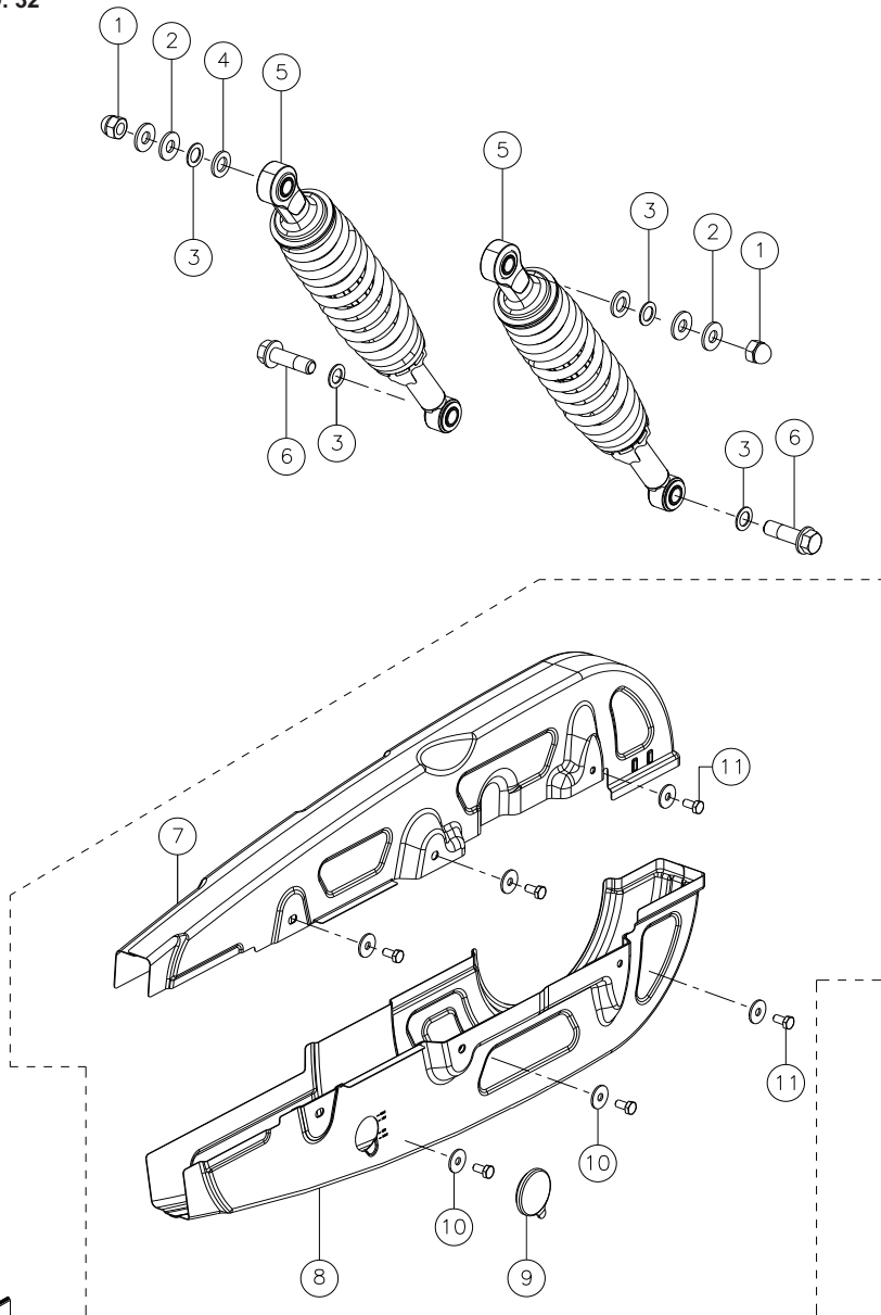
SHOCK ABSORBER & CHAIN CASE ASSY.
