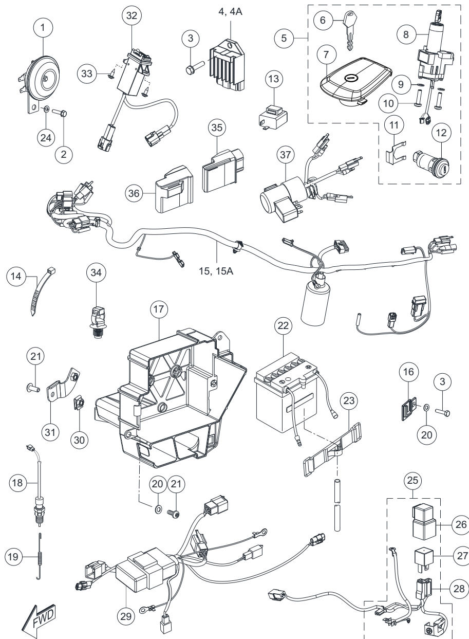
WIRING HARNESS ASSEMBLY
