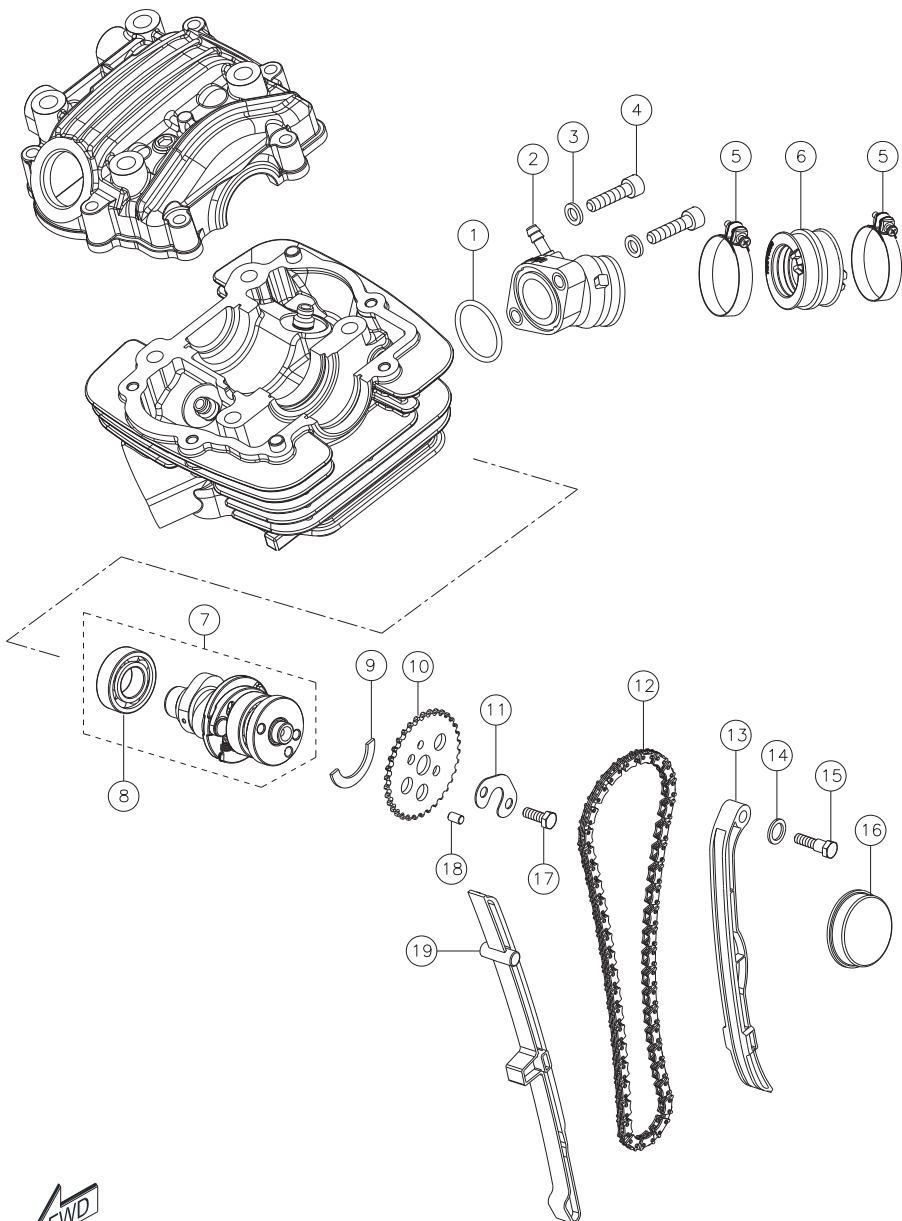
CAMSHAFT ASSEMBLY
