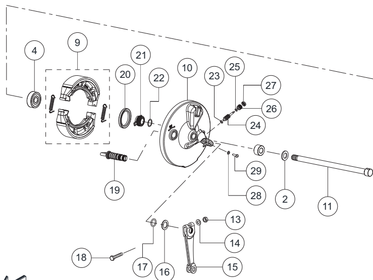
FRONT WHEEL ASSEMBLY
