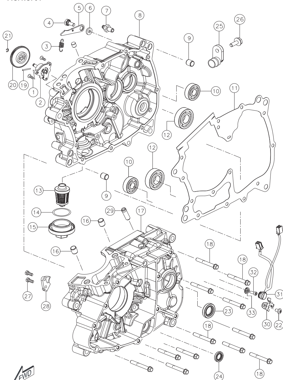
CRANKCASE ASSEMBLY
