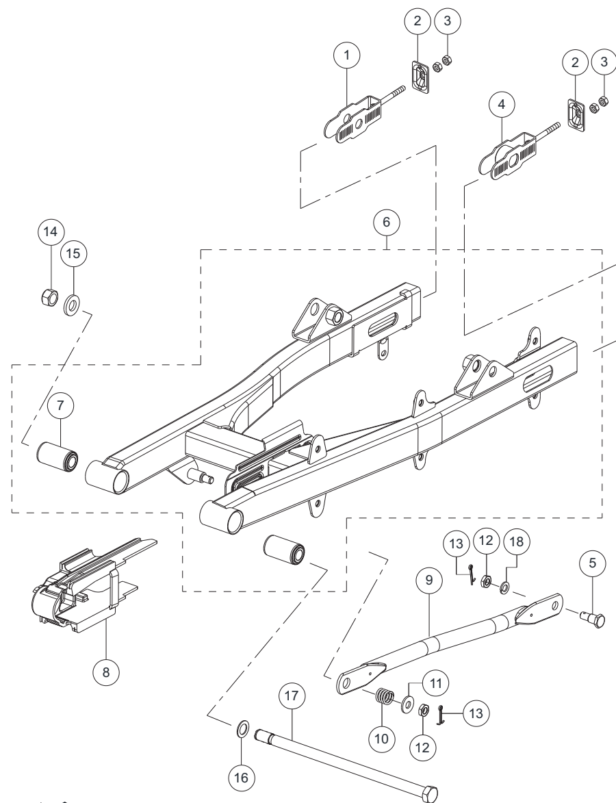
SWINGARM ASSEMBLY
