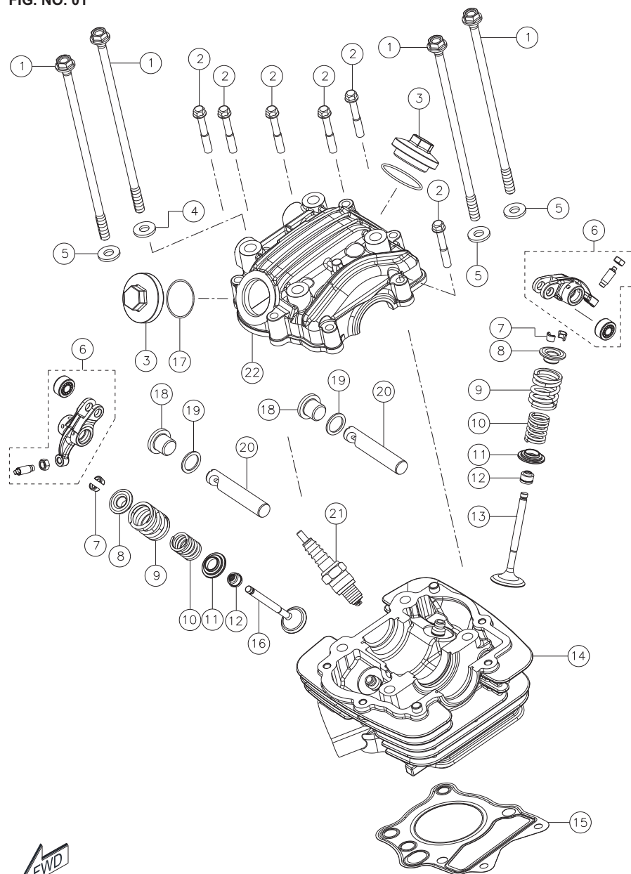
CYLINDER HEAD ASSEMBLY
