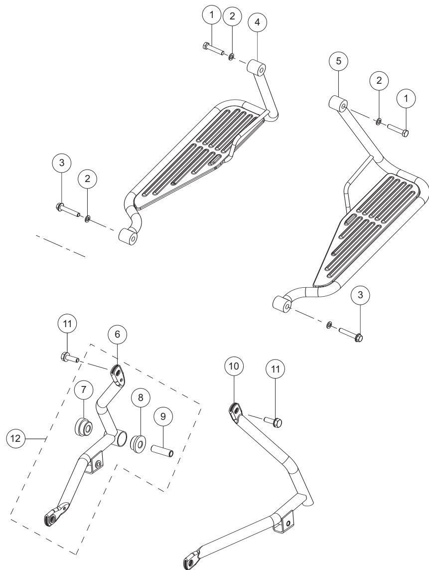
PILLION FOOTREST ASSEMBLY LH & RH
