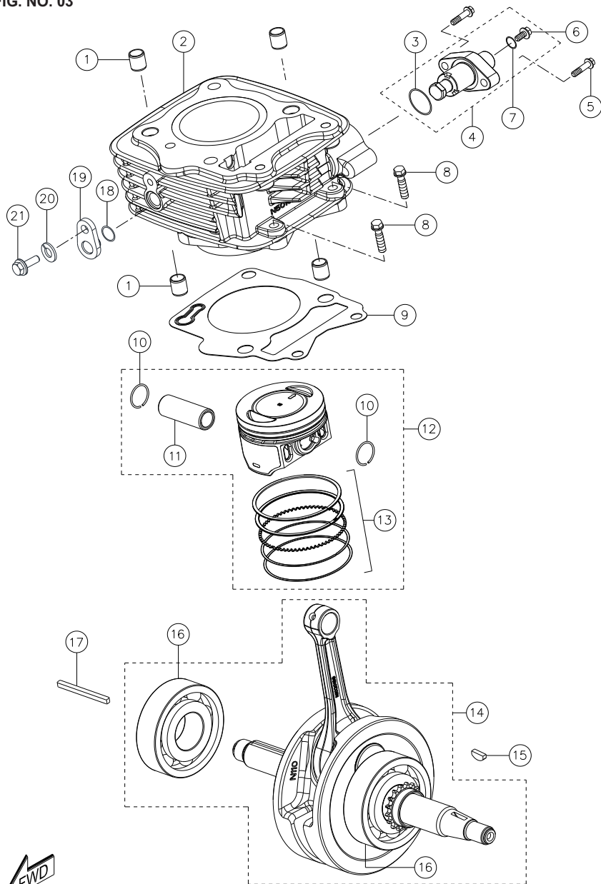
CYLINDER BLOCK &amp; CRANKSHAFT ASSY.
