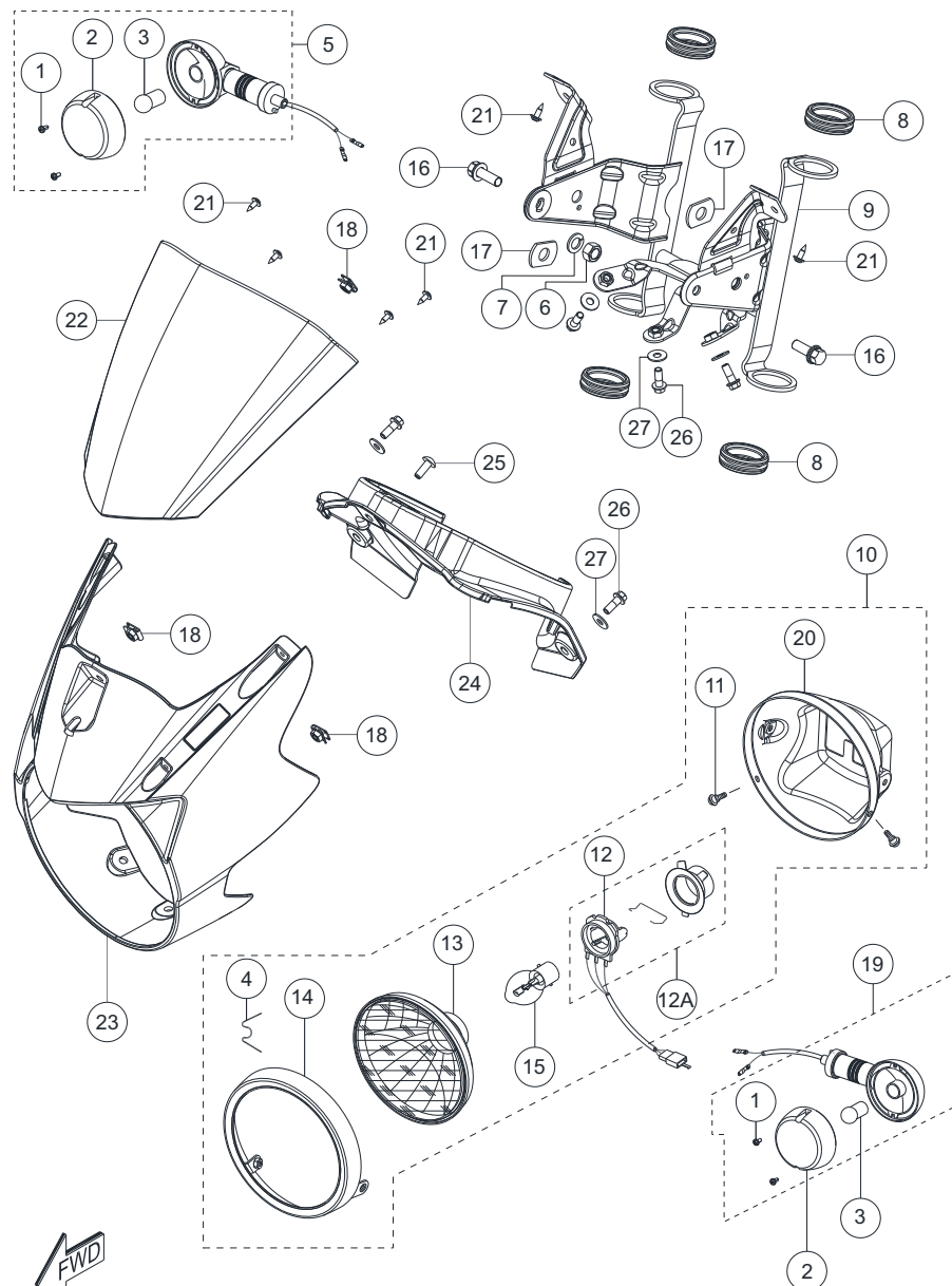
HEAD LAMP ASSEMBLY
