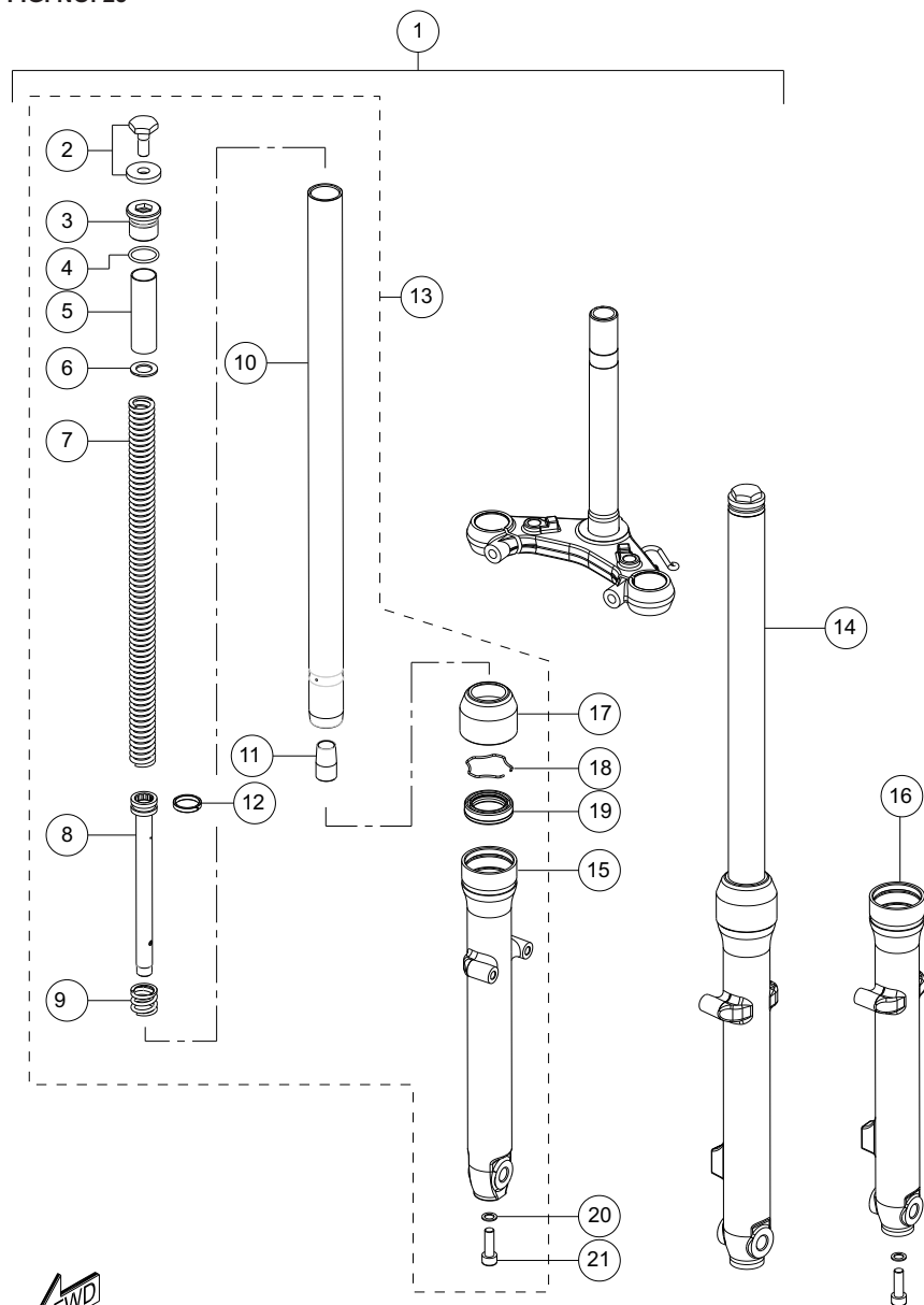
FRONT FORK ASSEMBLY
