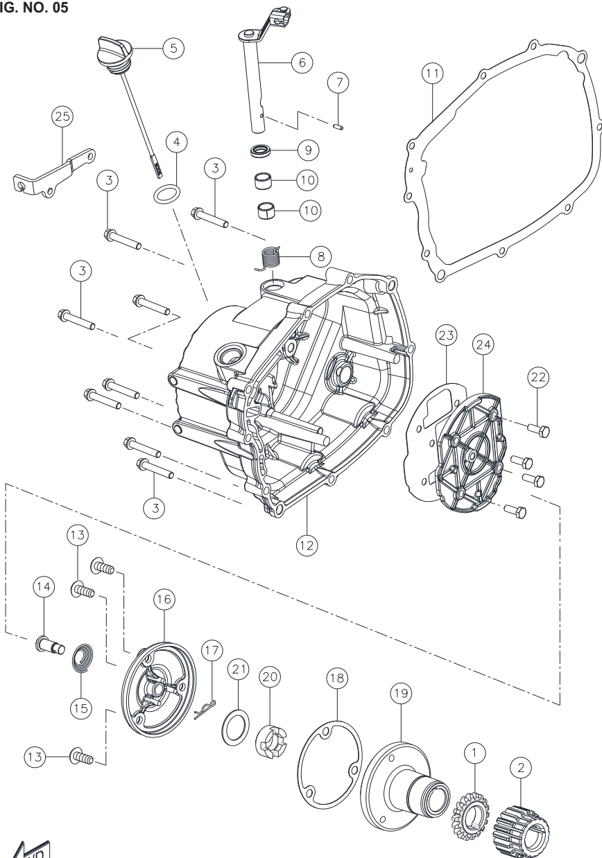
COVER CLUTCH ASSEMBLY
