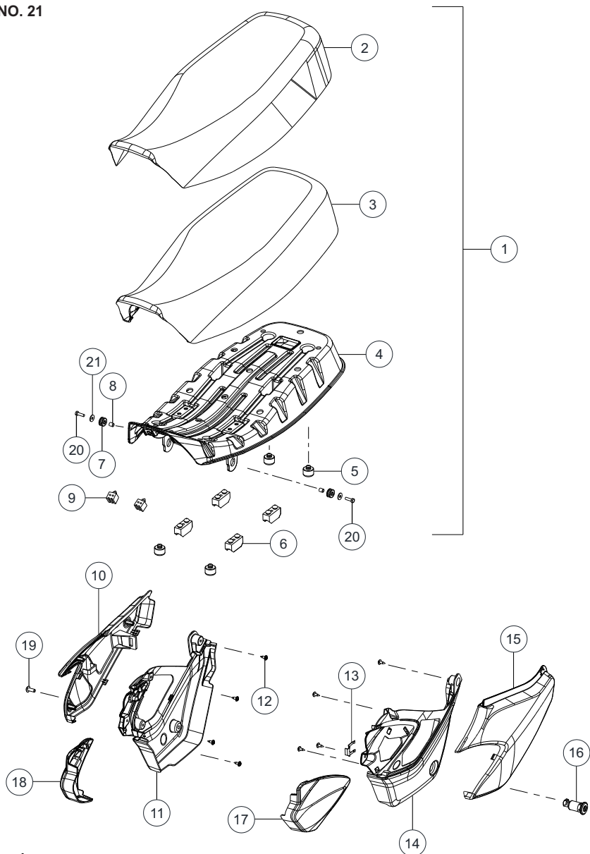
COVER FRAME &amp; SEAT ASSEMBLY
