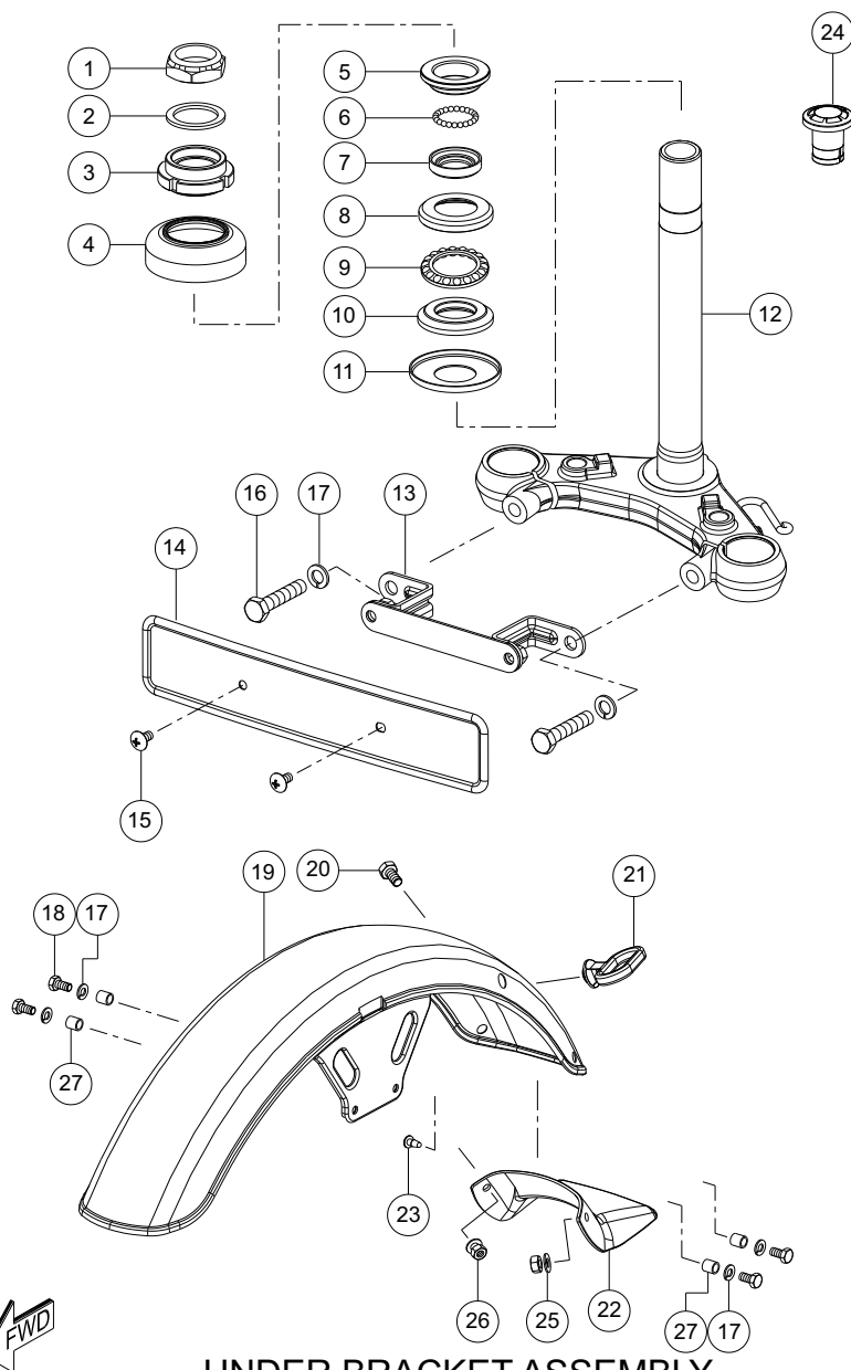
UNDER BRACKET ASSEMBLY
