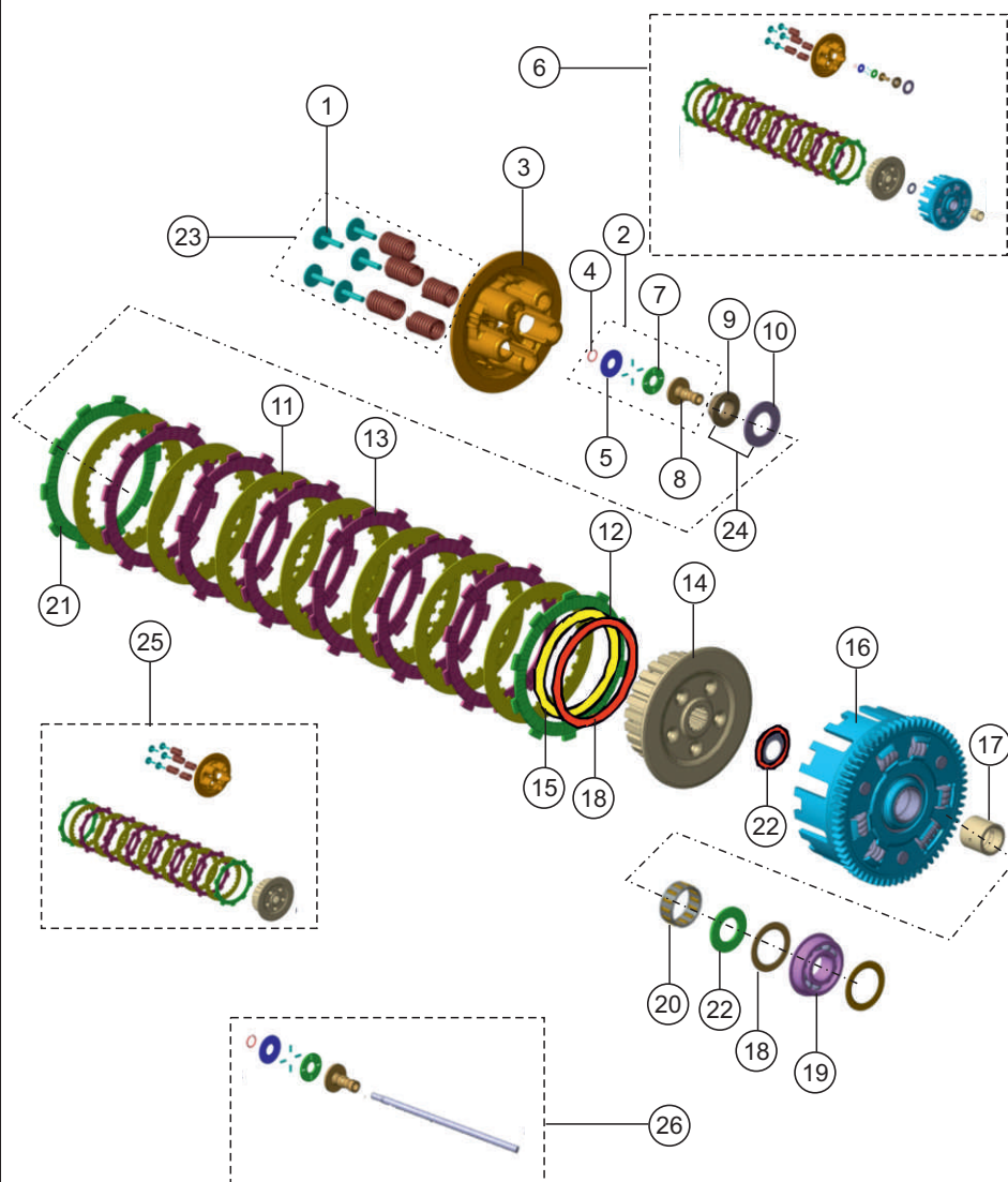
CLUTCH ASSEMBLY
