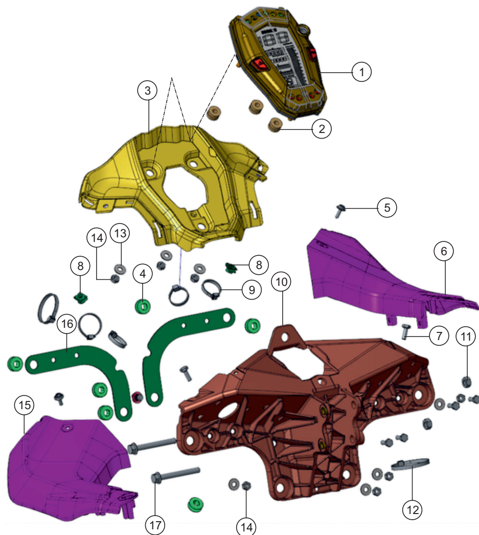
SPEEDOMETER ASSEMBLY
