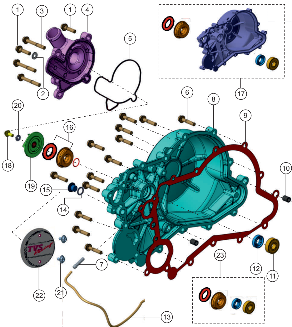
COVER CLUTCH ASSEMBLY
