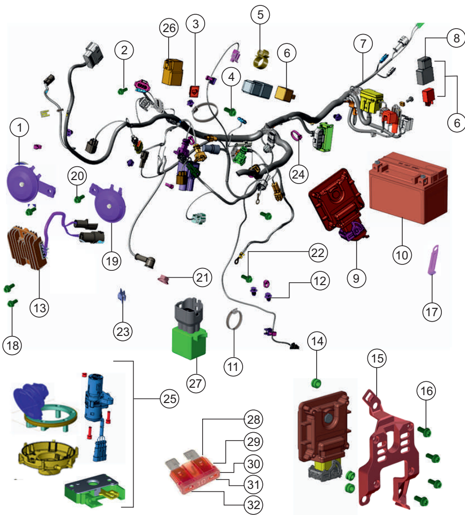
WIRING HARNESS ASSEMBLY
