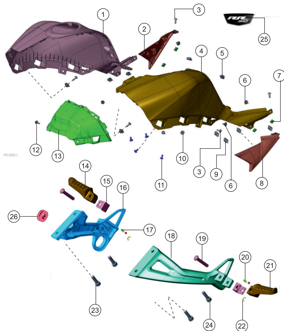
COVER FUEL TANK & PILLION FOOTREST ASSY.
