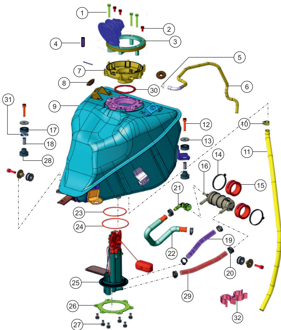
FUEL TANK ASSEMBLY
