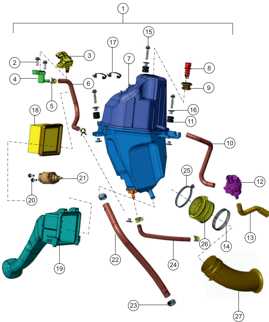
AIR CLEANER ASSEMBLY
