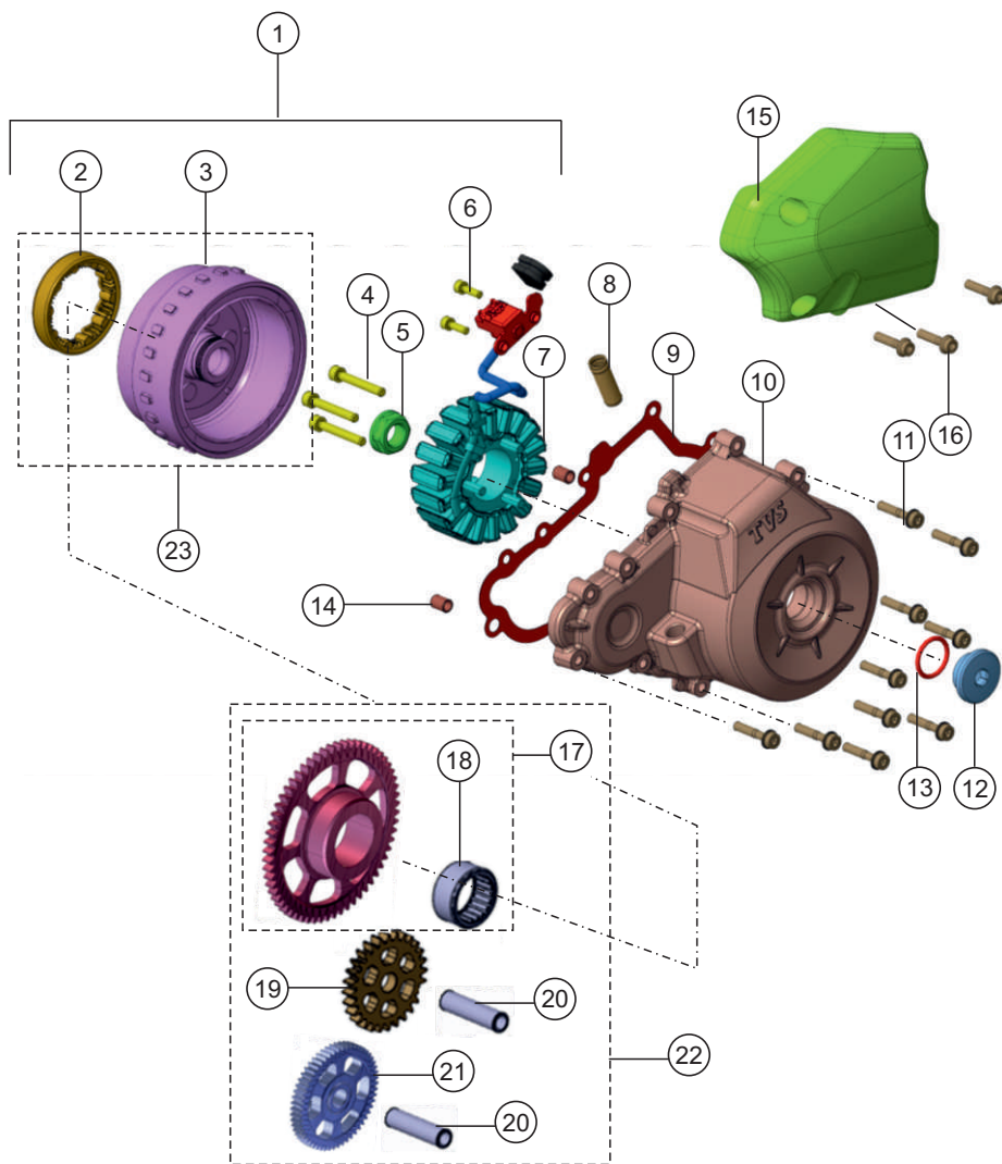
MAGNETO ASSEMBLY
