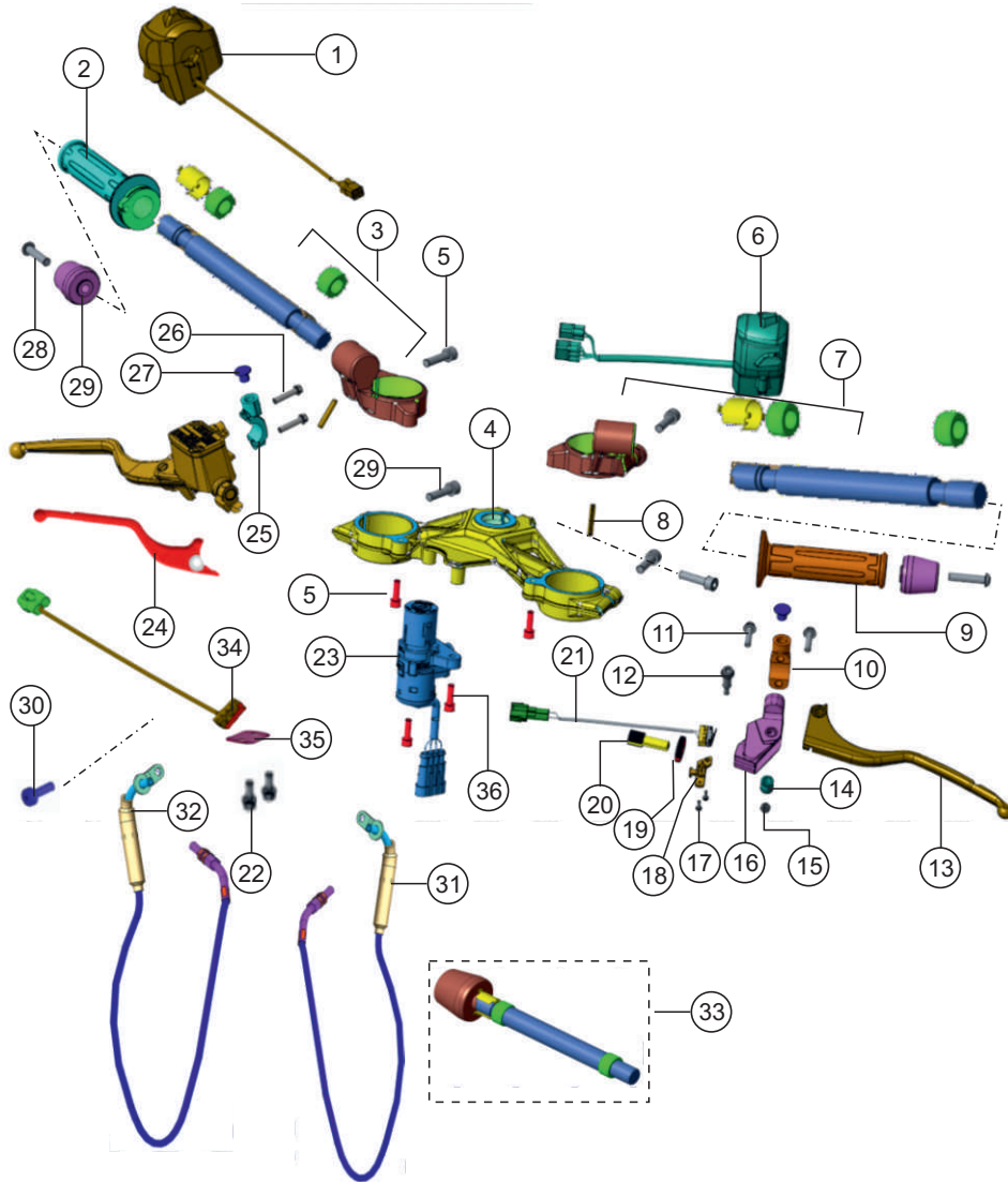
HANDLEBAR ASSEMBLY
