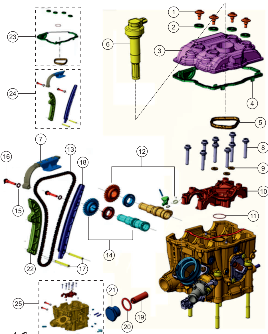
CYLINDER HEAD COVER ASSEMBLY
