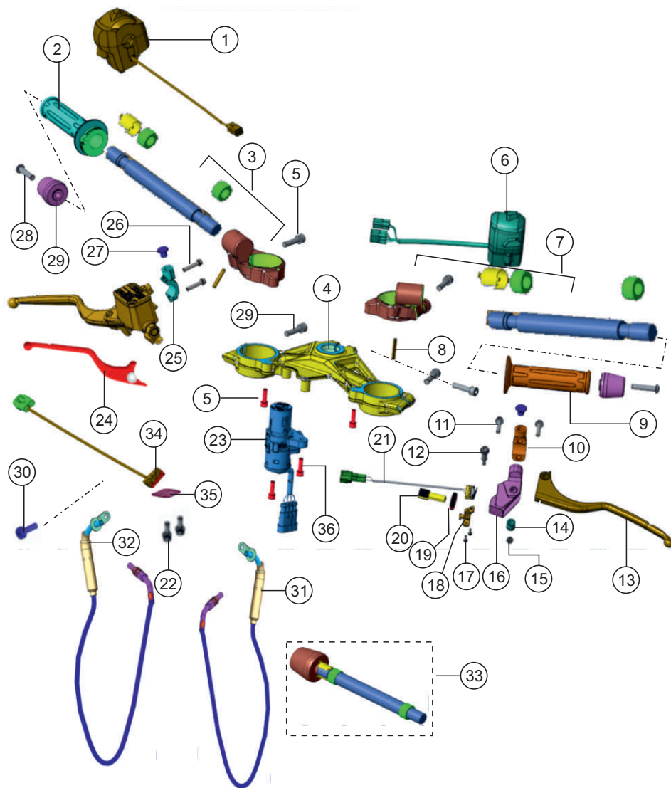
HANDLEBAR ASSEMBLY
