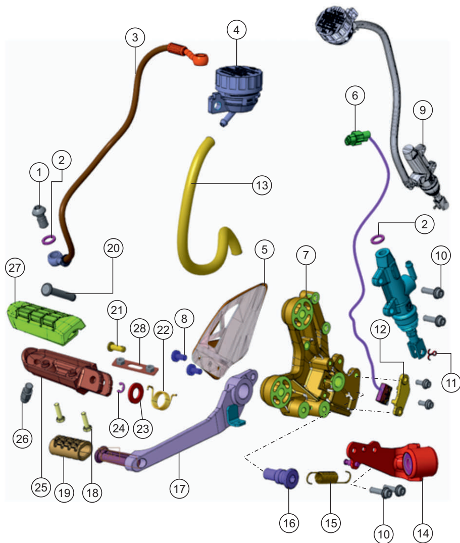
RIDER FOOTREST DISC ASSY. RH
