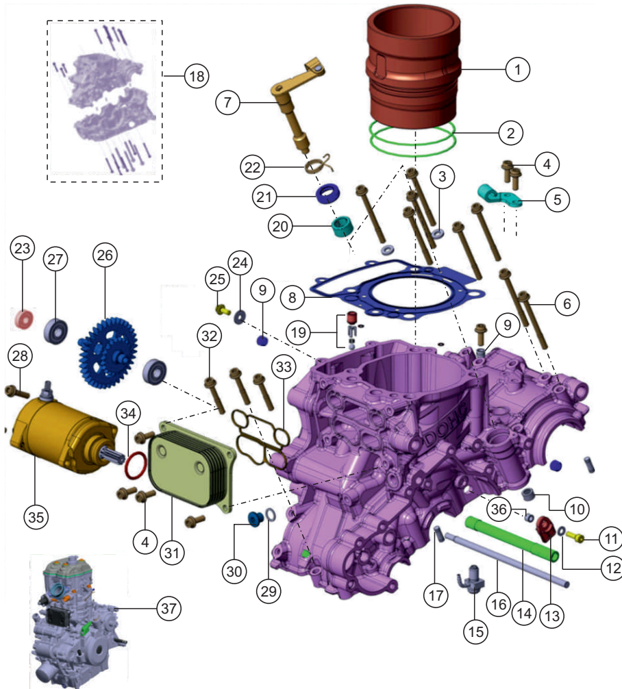
CRANKCASE ASSEMBLY STEP1 UPPER
