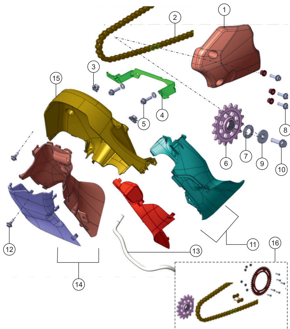
COVER ENGINE ASSEMBLY
