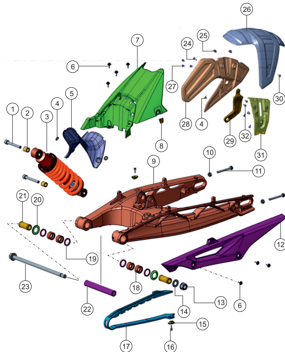
SWINGARM ASSEMBLY
