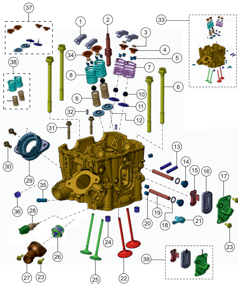
CYLINDER HEAD ASSEMBLY
