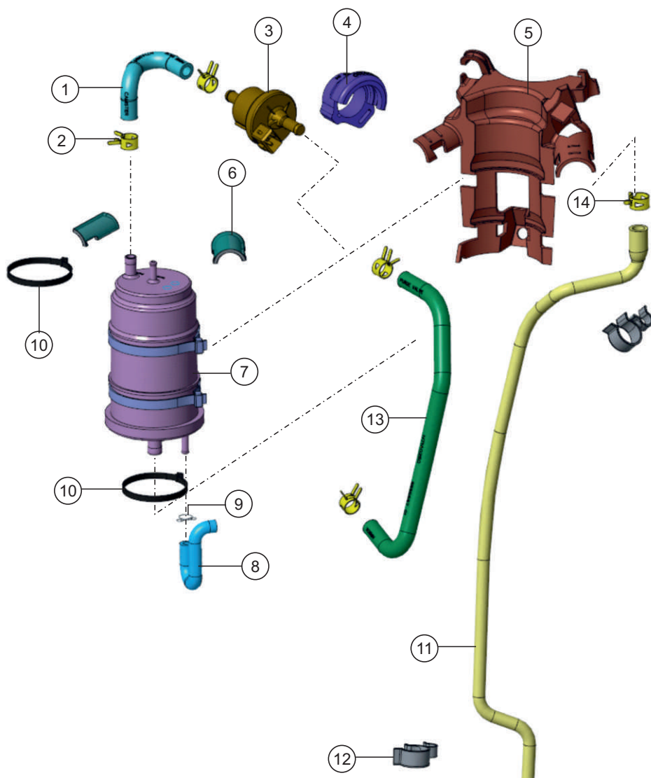
CANISTER ASSEMBLY
