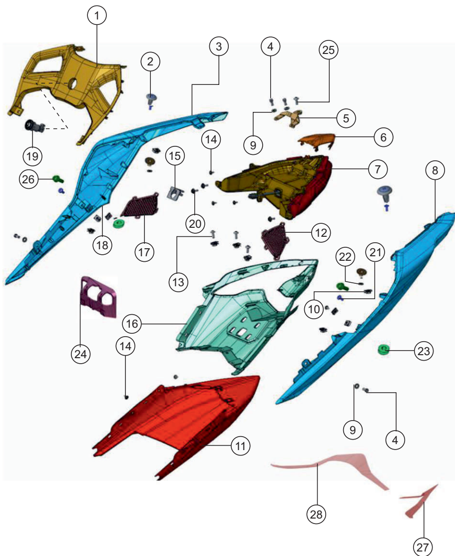
TAIL COVER & TAIL LAMP ASSY.
