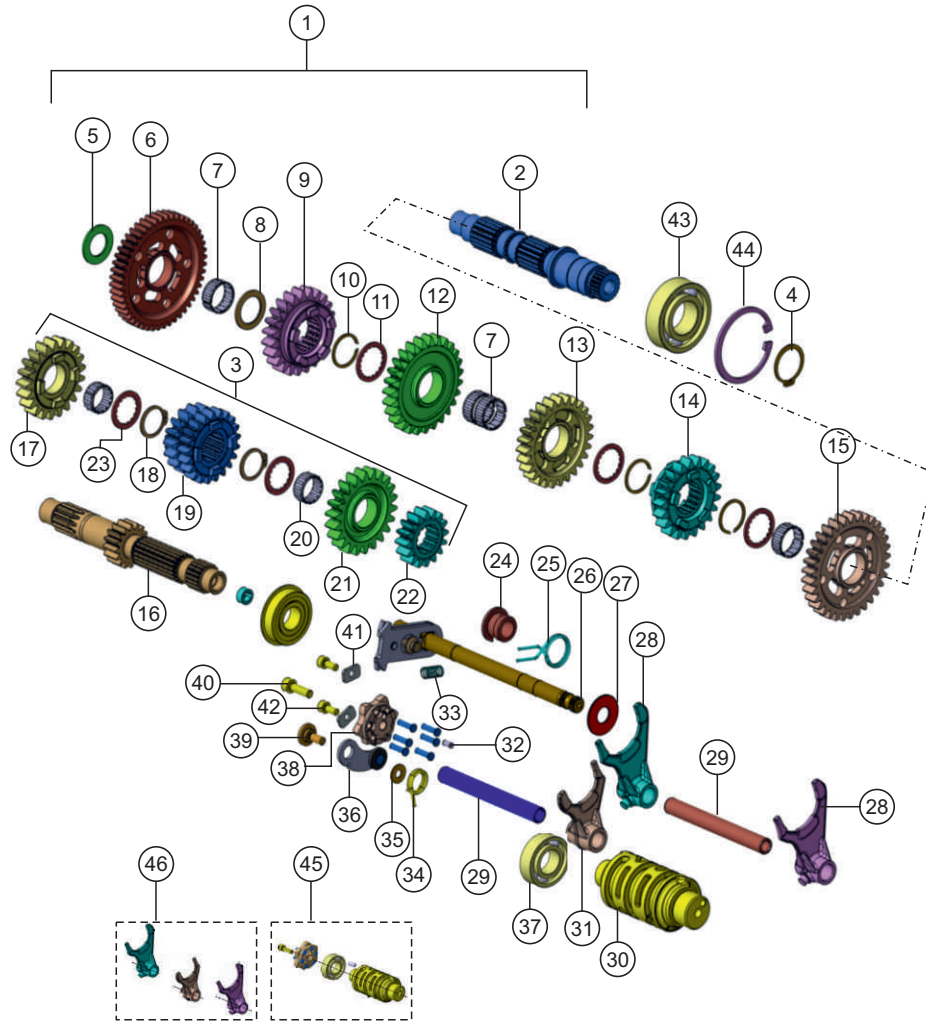
GEAR AND GEARSHIFT ASSEMBLY
