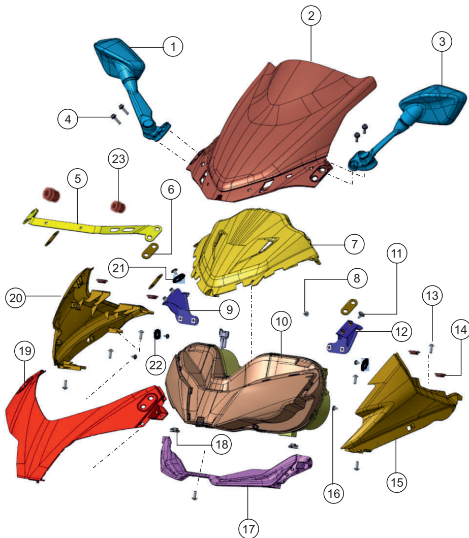
HEAD LAMP ASSEMBLY
