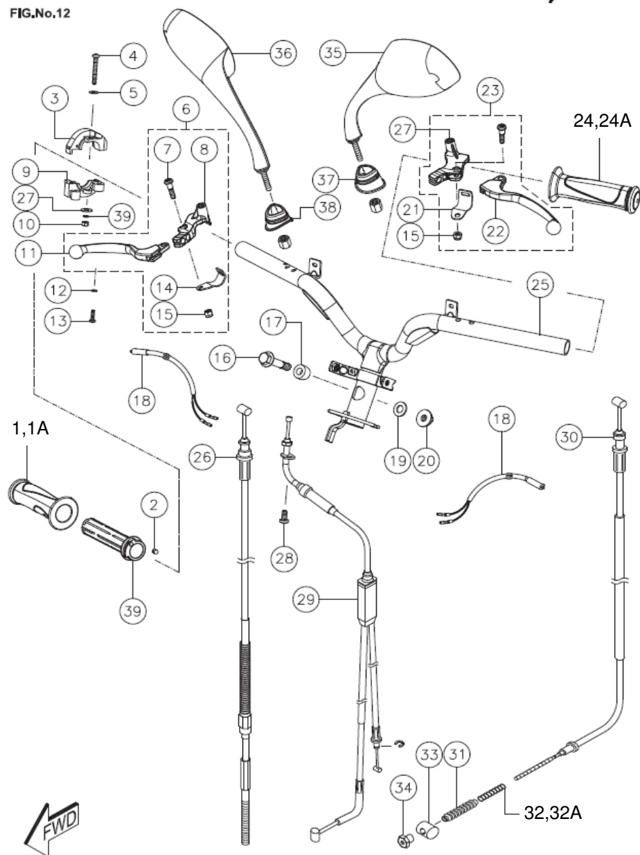
HANDLEBAR & CABLE ASSEMBLY
