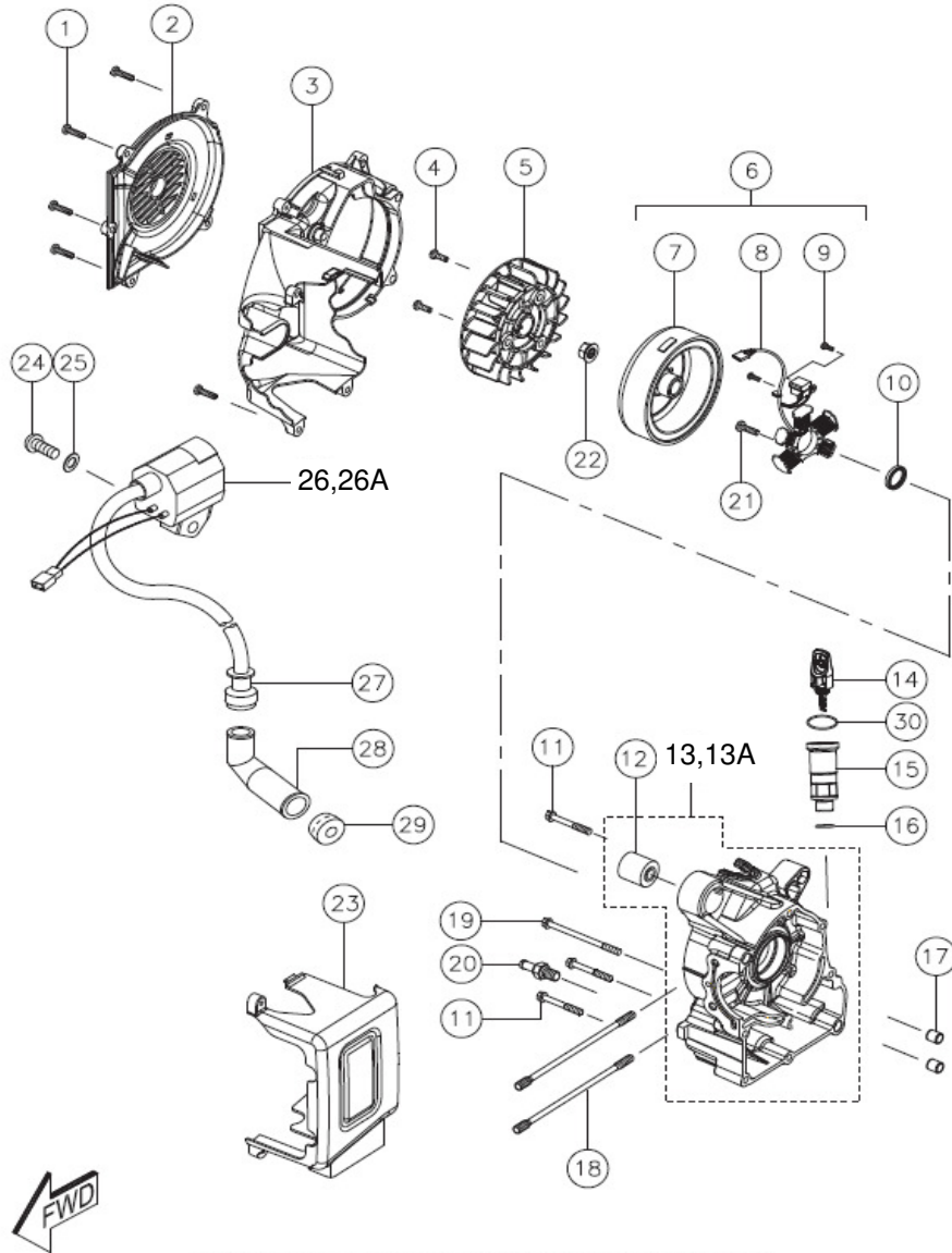
CRANKCASE RH & MAGNETO ASSEMBLY
