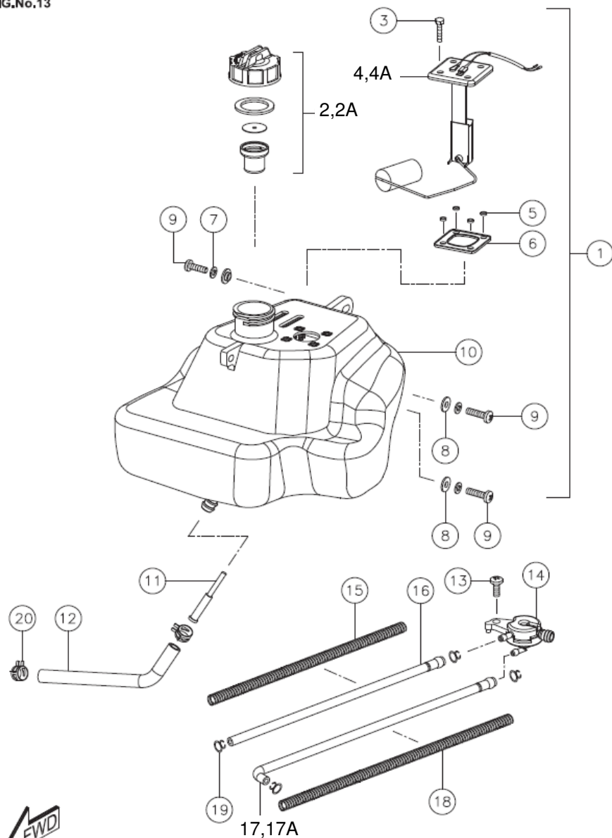
FUEL TANK & AUTO FUEL COCK ASSEMBLY
