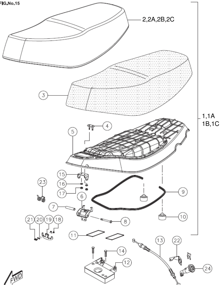
SEAT ASSEMBLY
