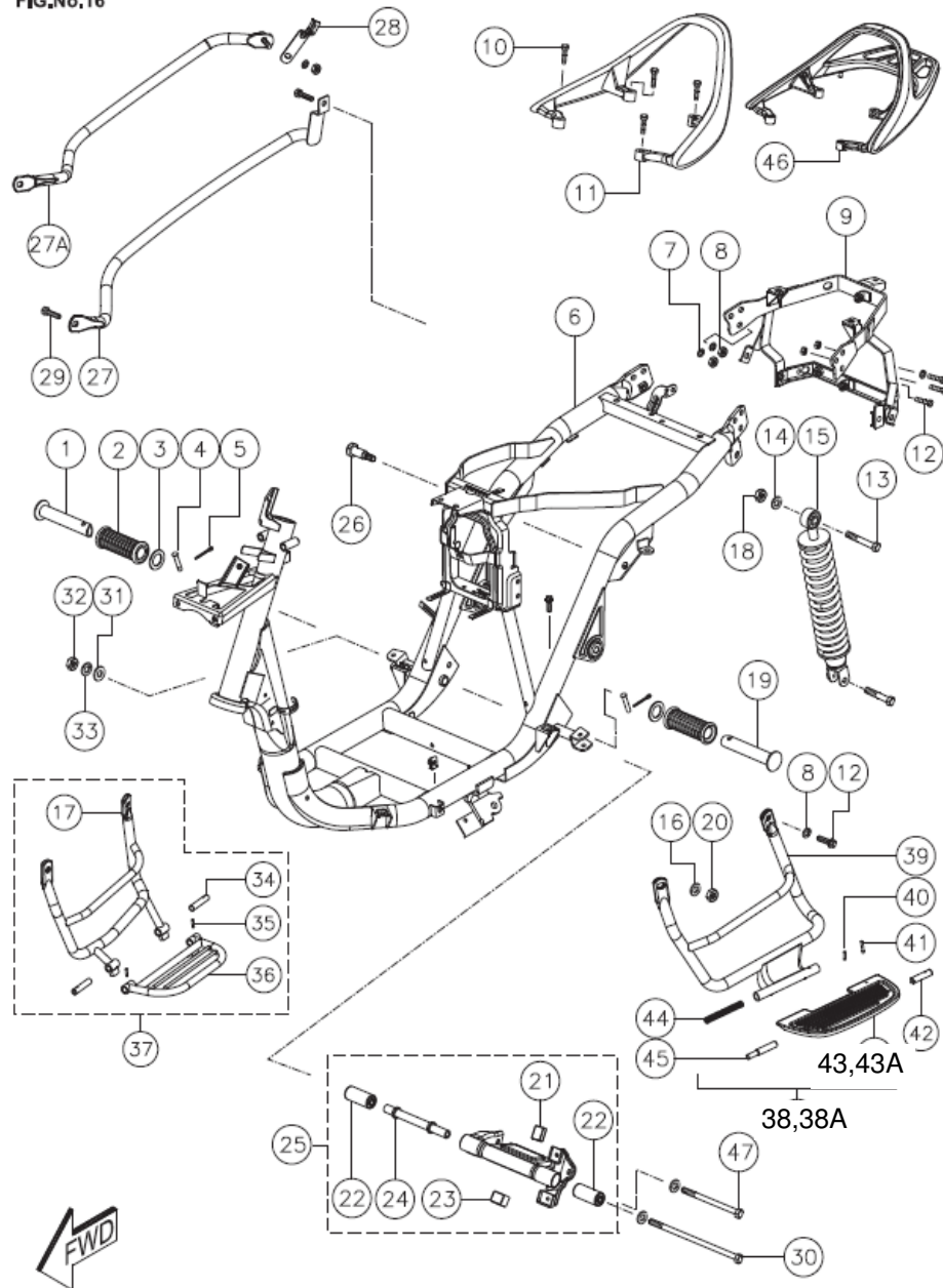
FRAME & FOOTREST ASSY.
