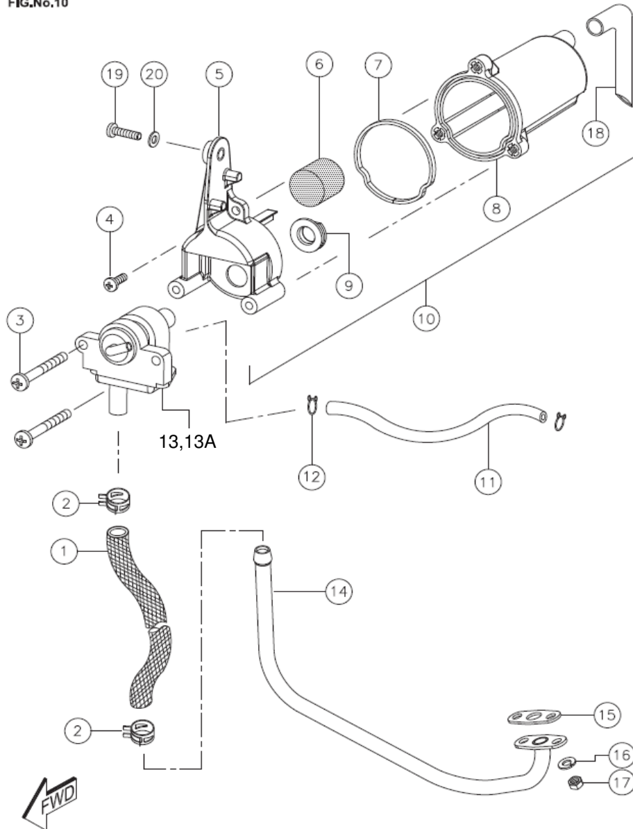
SECONDARY AIR INJECTION ASSY.
