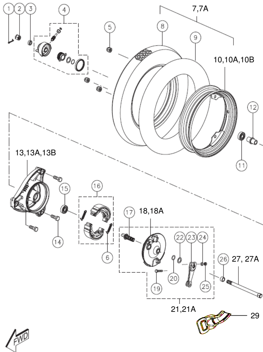
FRONT WHEEL ASSEMBLY
