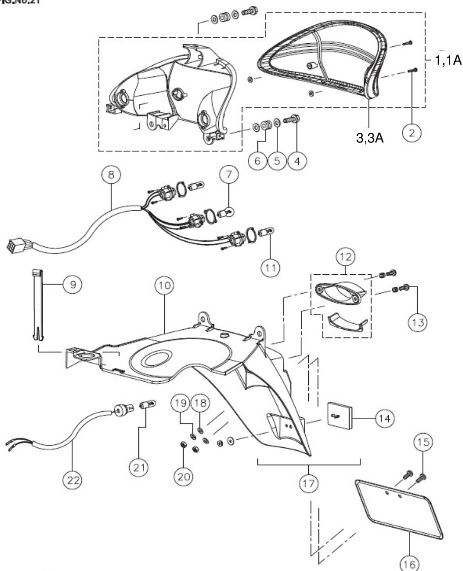
TAIL LAMP & REAR FENDER ASSY.
