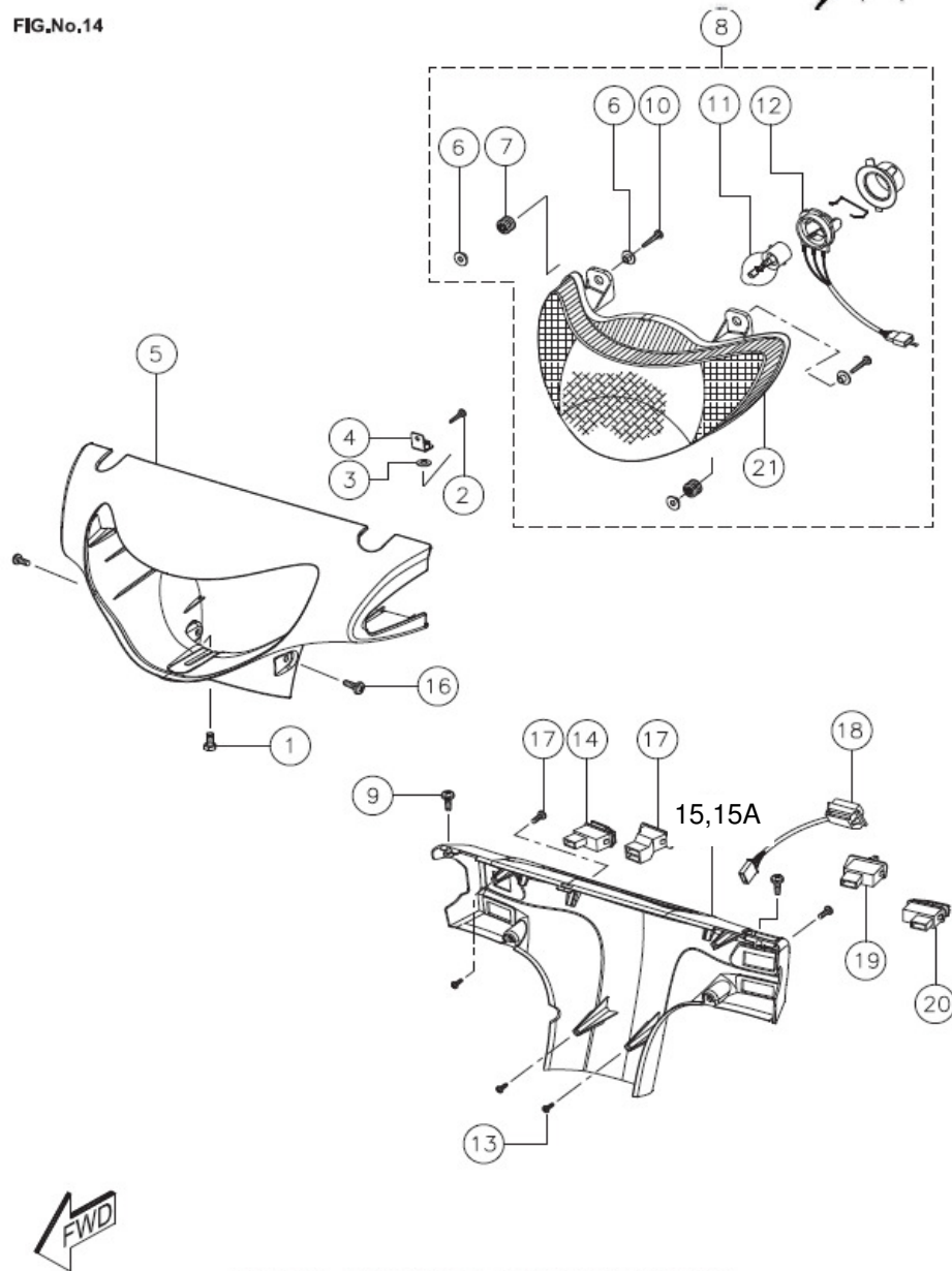
HEAD LAMP ASSY. & HOUSING ASSY.
