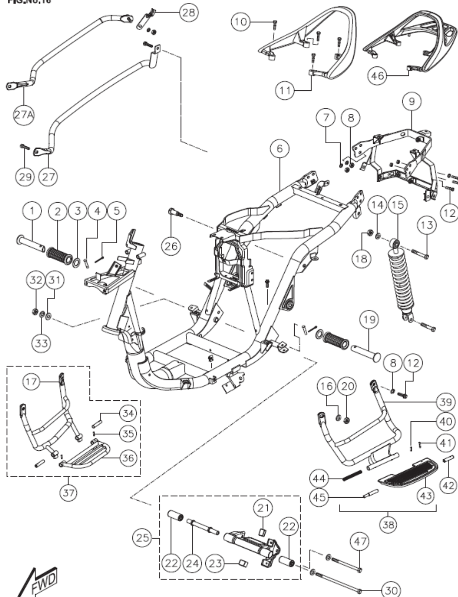
FRAME &amp; FOOTREST ASSY.
