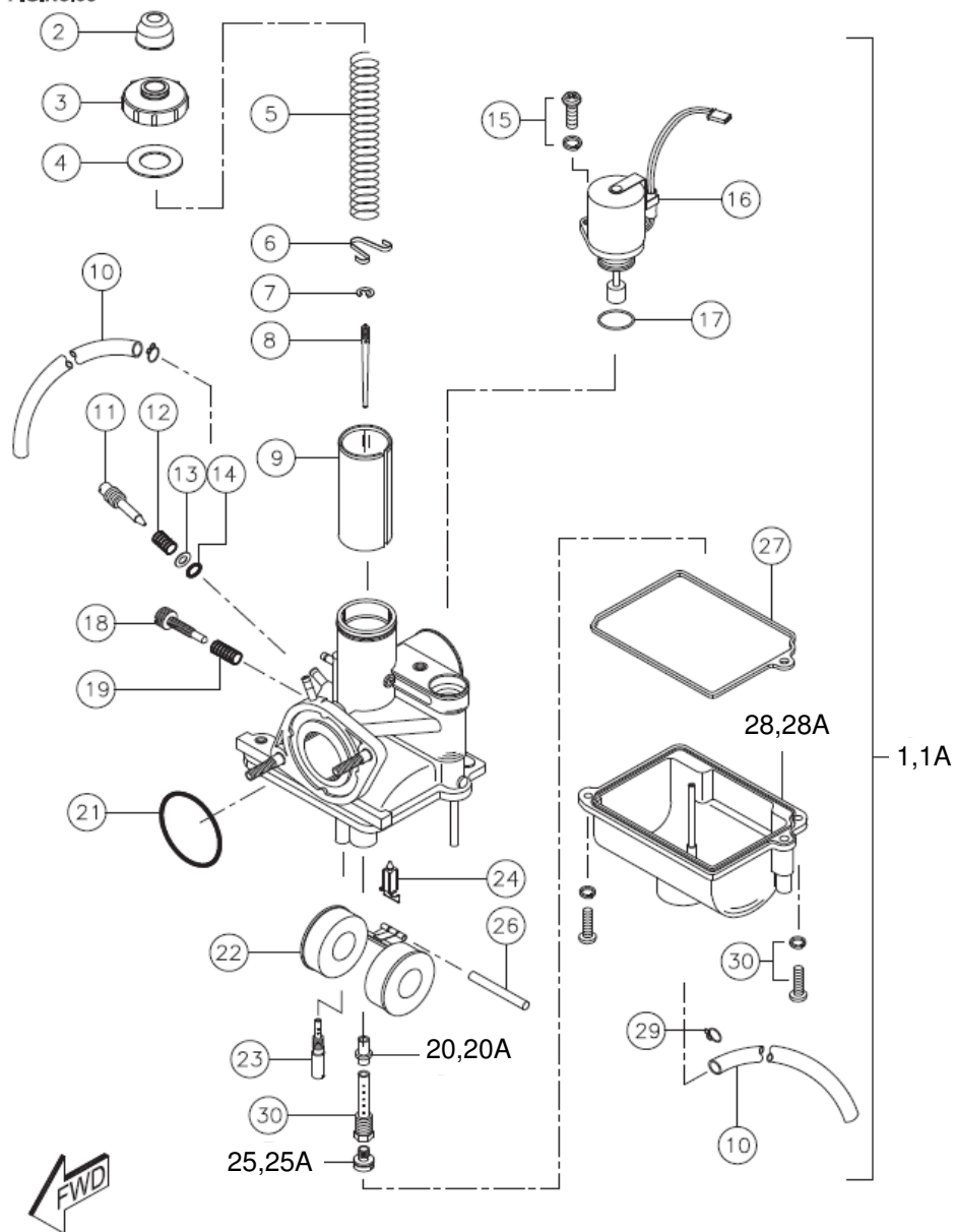
CARBURETTOR ASSEMBLY
