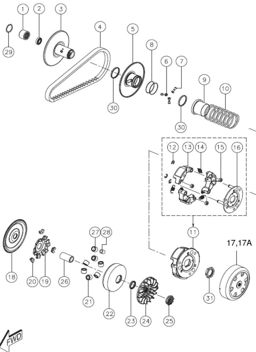
CLUTCH &amp; VARIAMATIC ASSEMBLY
