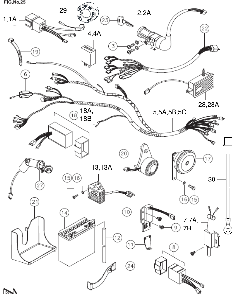
WIRING HARNESS & BATTERY ASSY.
