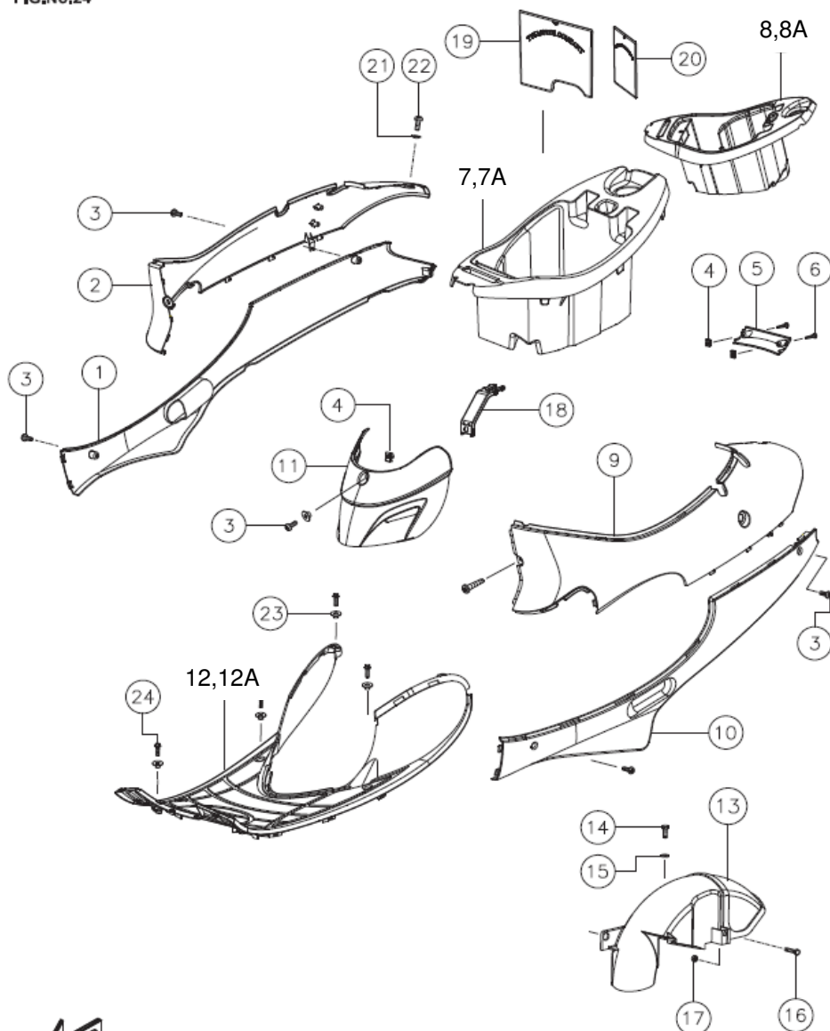
PANEL SIDE LH, RH & REAR MUDGUARD
