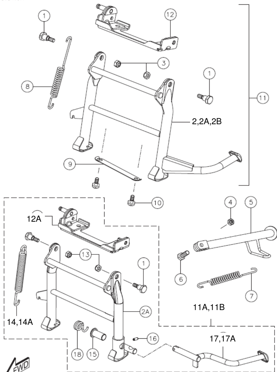
CENTER STAND &amp; PROP STAND ASSY.
