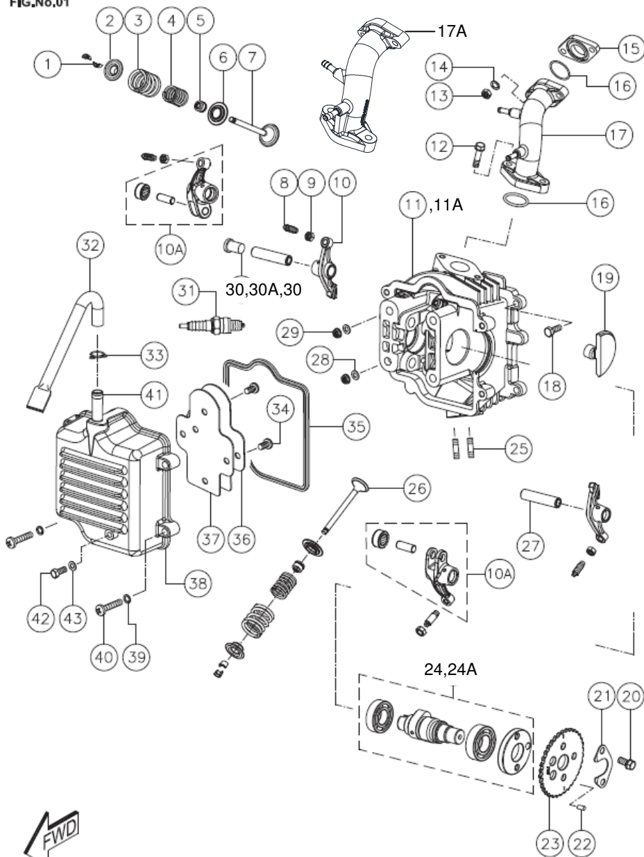
CYLINDER HEAD ASSEMBLY
