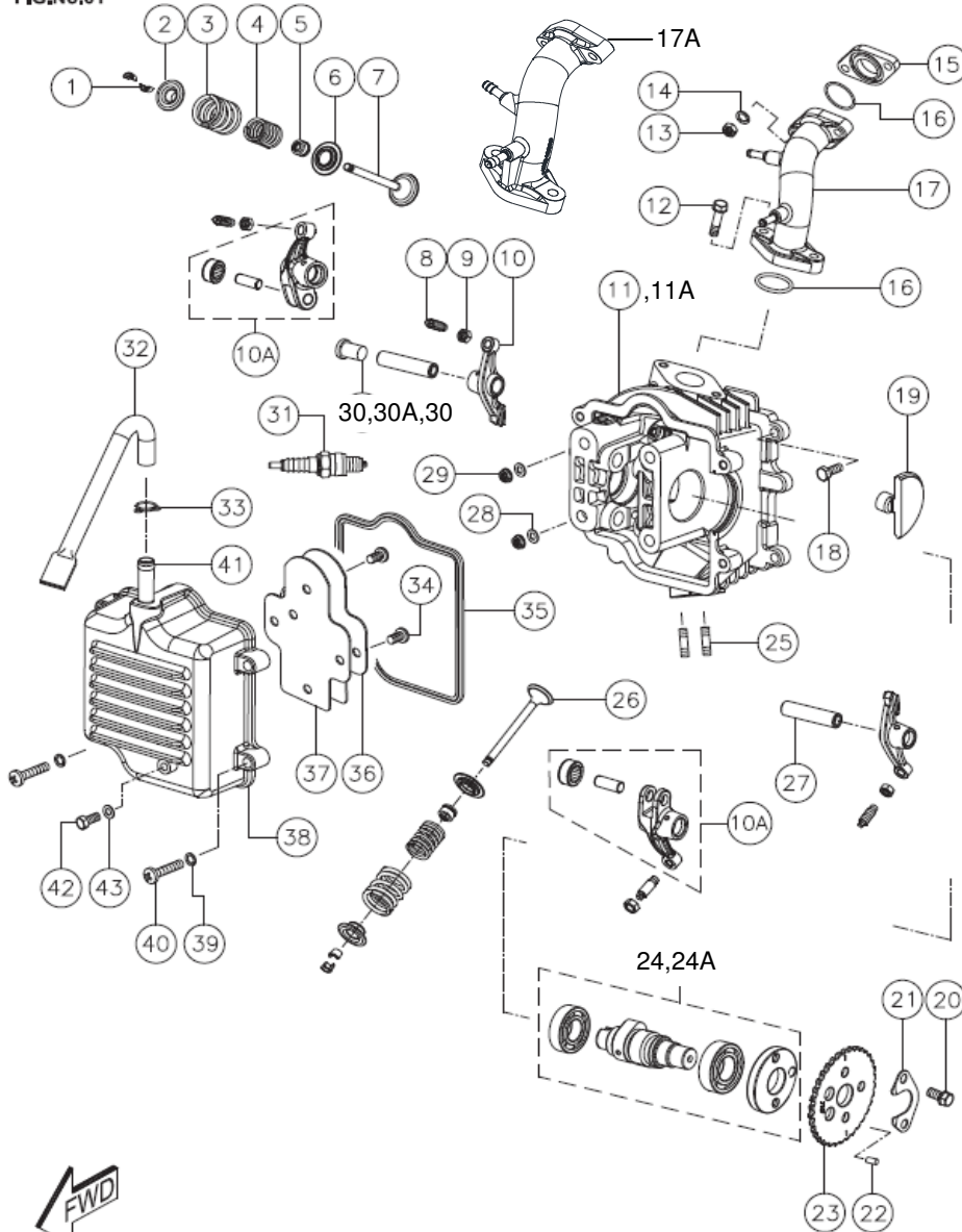
CYLINDER HEAD ASSEMBLY
