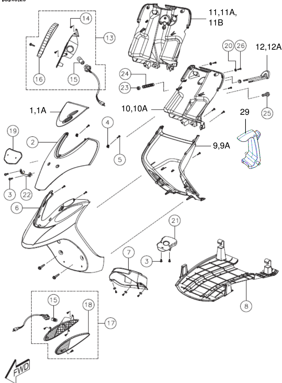
FRONT & REAR PANEL ASSEMBLY
