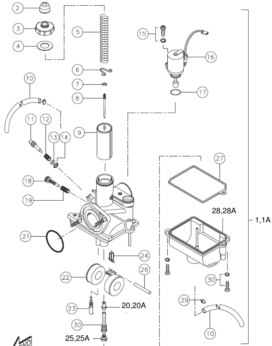
CARBURETTOR ASSEMBLY
