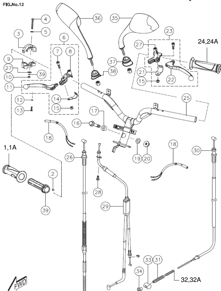
HANDLEBAR &amp; CABLE ASSEMBLY
