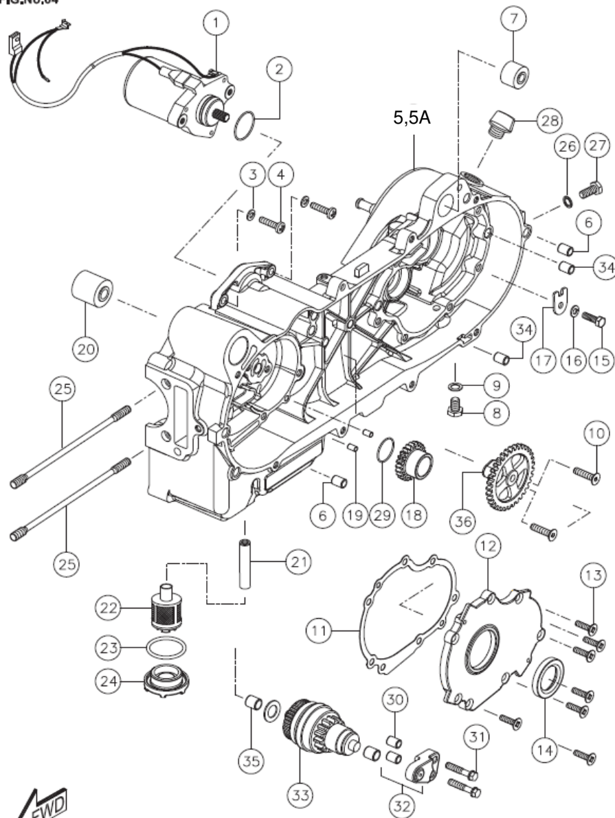
CRANKCASE LH & OIL PUMP ASSY.
