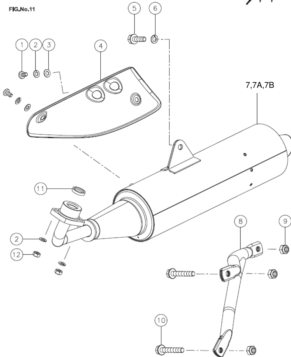
MUFFLER ASSEMBLY
