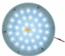
FPS Code : LRW06A/LRW06B LED Light Assembly - 12/24V - 6 Watt Round - White Color
