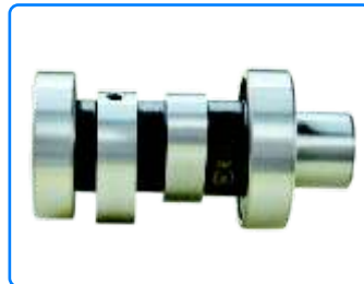
PART NO. : 520AM00362 APPLICATION : CAM SHAFT SUITABLE FOR : BAJAJ PLATINA STD. PACK : 10
