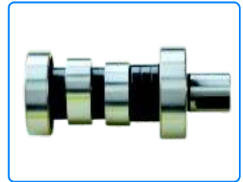
PART NO. : 520AM00363 APPLICATION : CAM SHAFT SUITABLE FOR : BAJAJ PULSAR-135LS/ DISCOVER-125ST STD. PACK : 10
