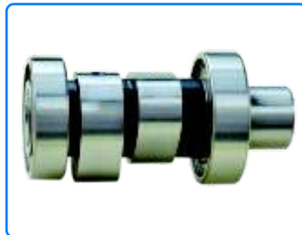
PART NO. : 520AM00359 APPLICATION : CAM SHAFT SUITABLE FOR : BAJAJ CT-100 STD. PACK : 10
