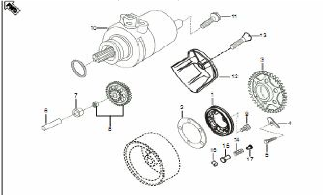
Plate No. 23 : STARTER ASSEMBLY (FOR SELF START)
