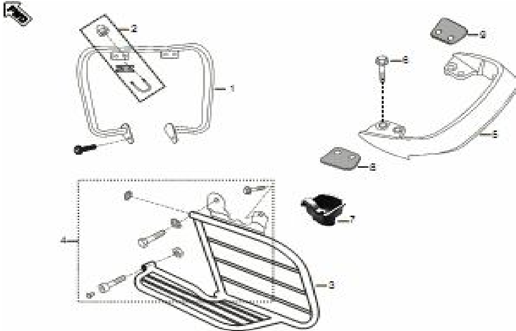
Plate No. 50 : ACCESSORIES / GRAB HANDLE
