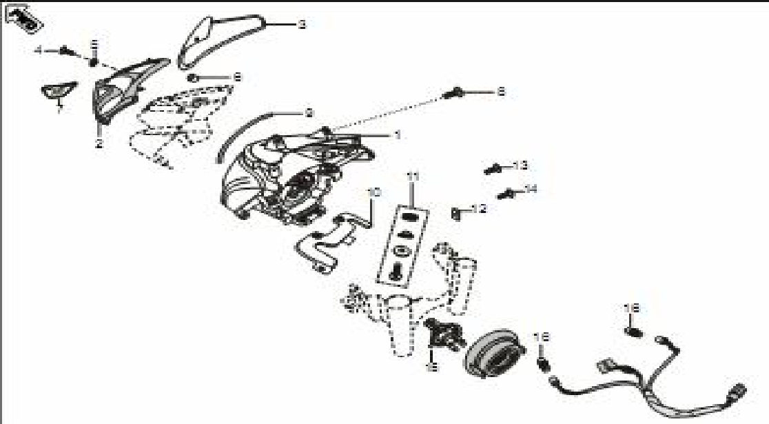
Plate No. 45 : HEAD LAMP & FAIRING
