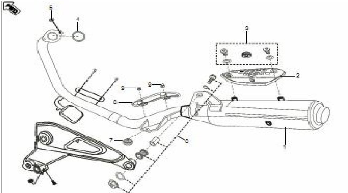
Plate No. 19 : SILENCER ASSLY.
