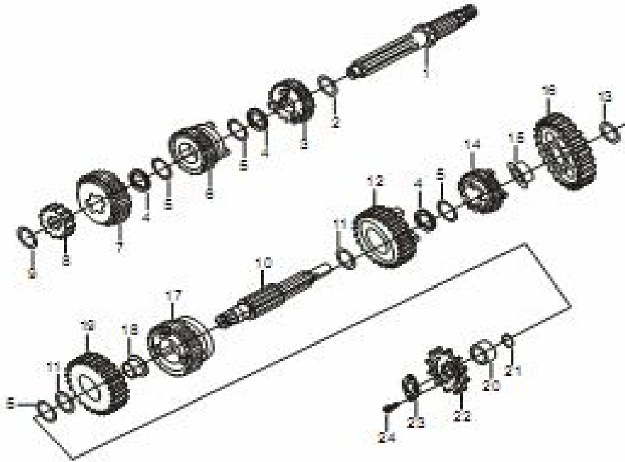
Plate No. 8 : TRANSMISSION
