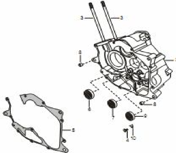
Plate No. 11: ENGINE ASSY & CRANK CASE RH
