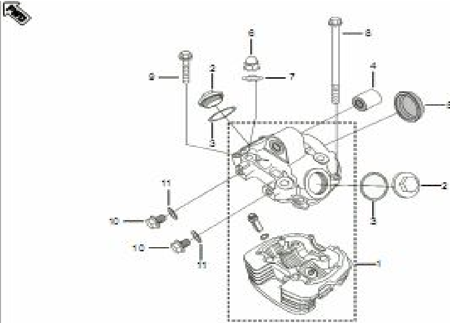
Plate No. 1 : COVER CYLINDER HEAD
