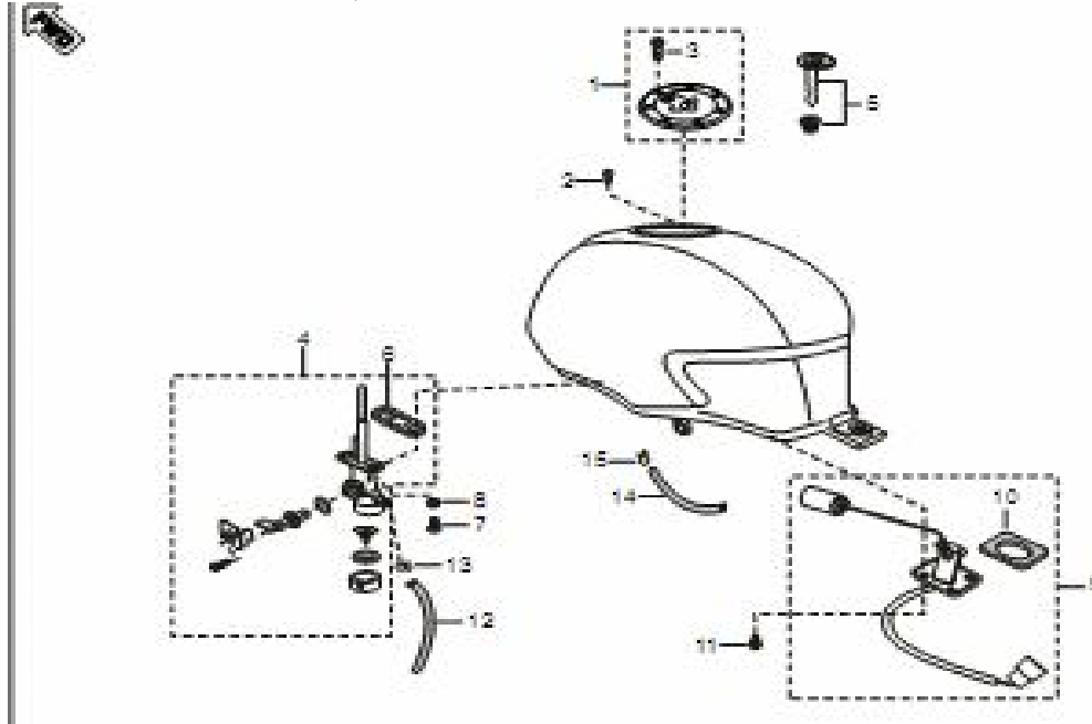
Plate No. 40 : PETROL COCK, CAP TANK & GAUGE FUEL
