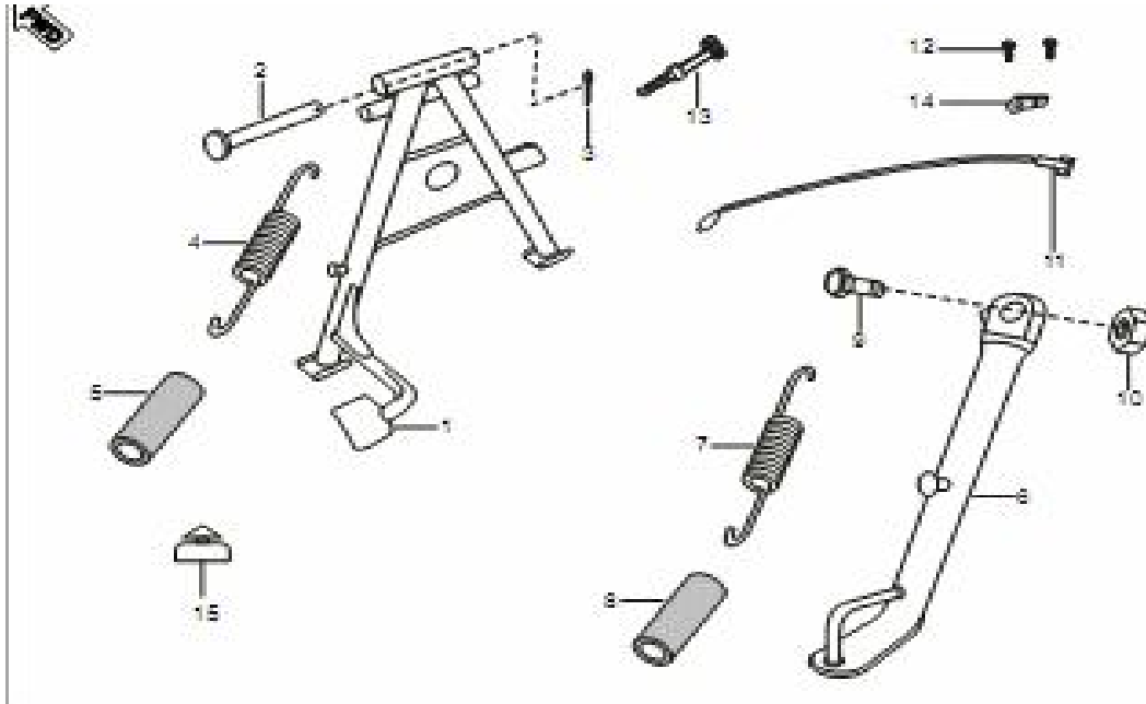
Plate No. 30 : STAND ASSEMBLY
