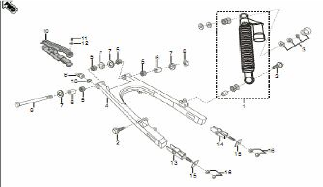
Plate No. 26 : SWING ARM / REAR SHOCK ABSORBER
