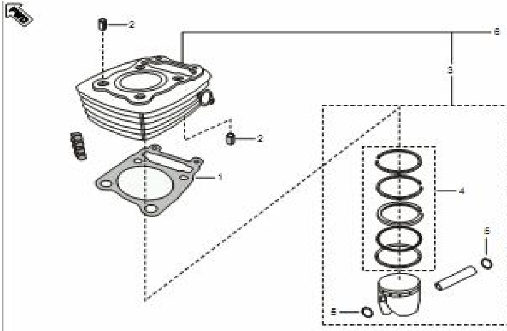
Plate No. 5 : CYLINDER AND PISTON
