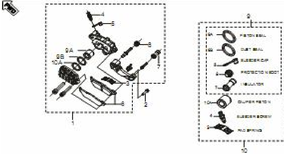
Plate No. 34 : FRONT DISC BRAKE
