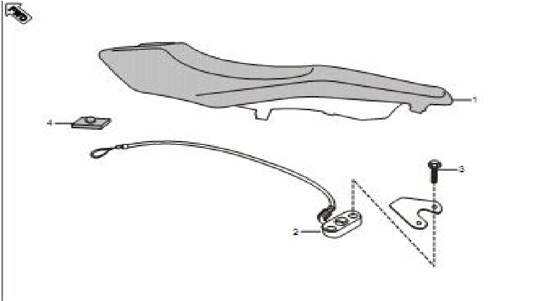
Plate No. 20 : SEAT ASSLY. / SEAT LOCK
