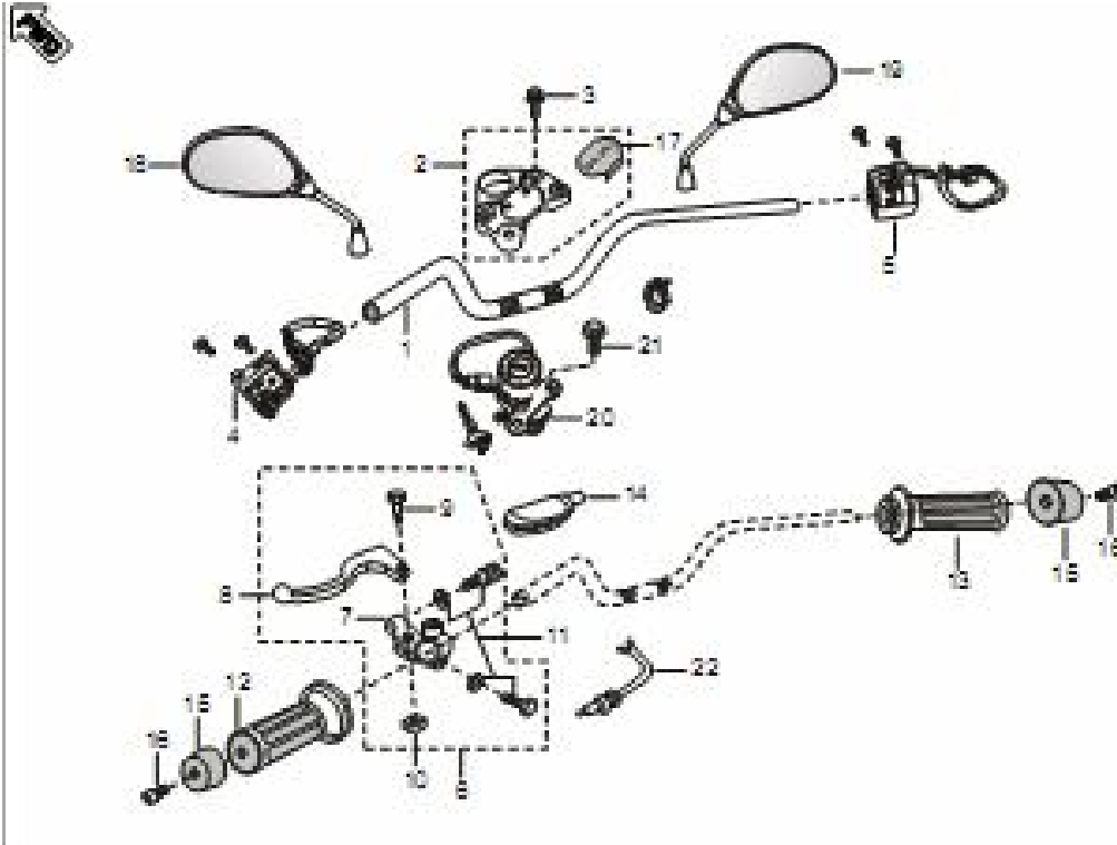
Plate No. 37 : HANDLE BAR
