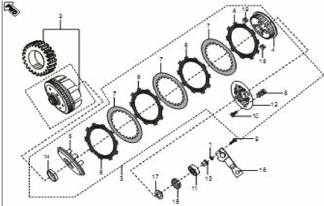
Plate No. 15 : CLUTCH
