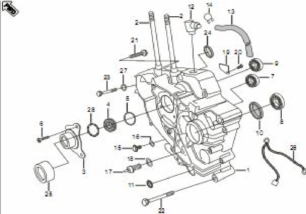
Plate No. 12 : CRANKCASE LH
