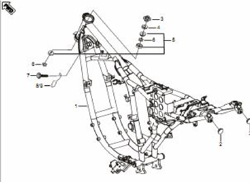
Plate No. 25 : FRAME & FRAME FITTINGS
