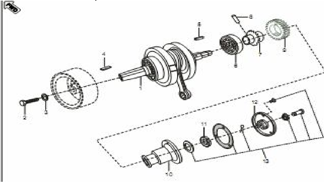
Plate No. 6 : Crank shaft assy
