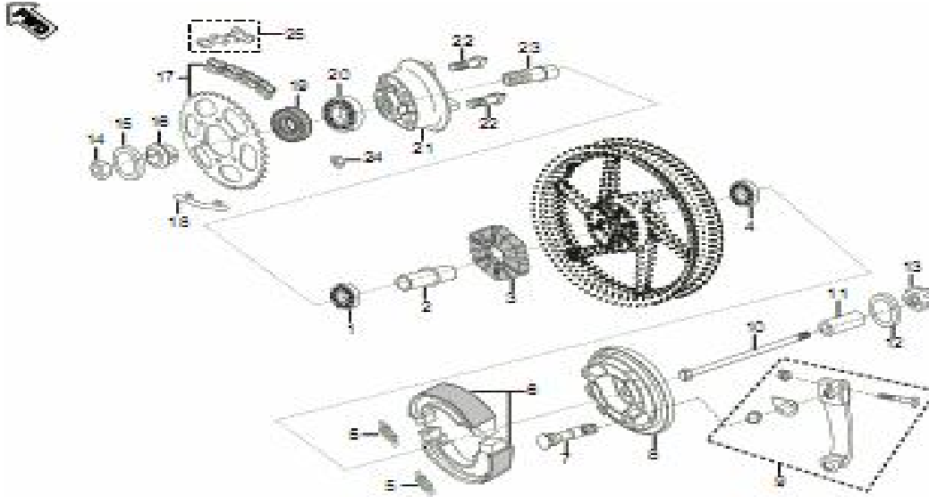
Plate No. 35 : REAR HUB
