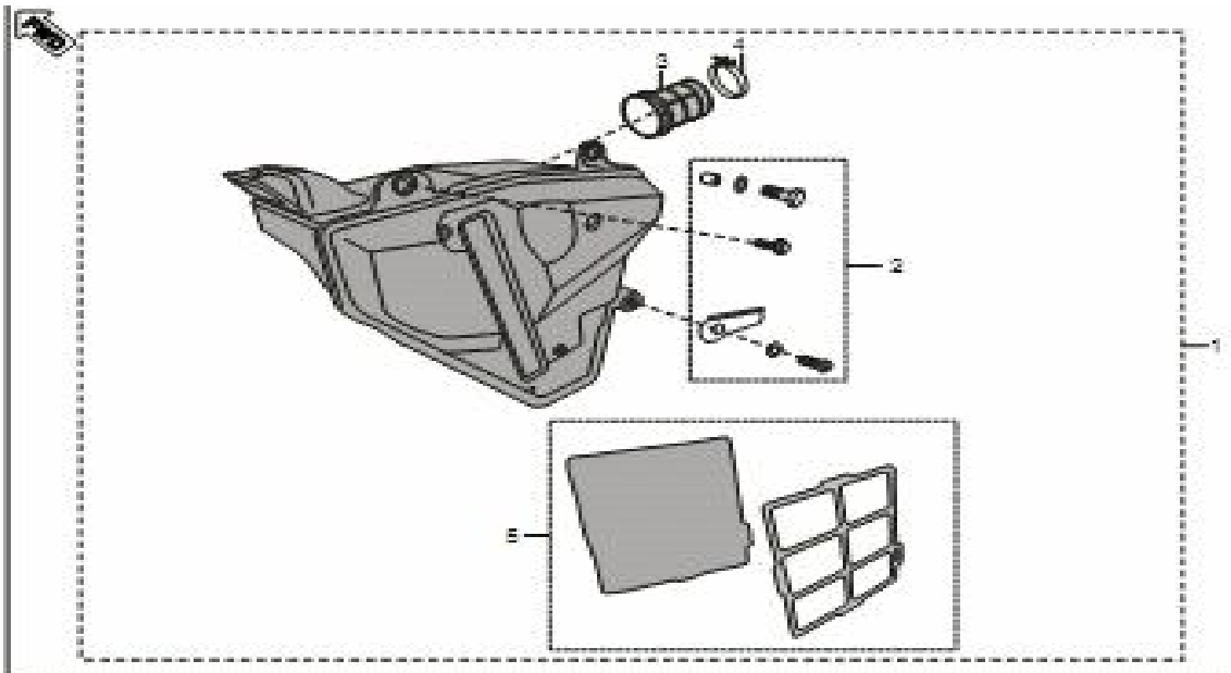
Plate No. 18 : AIR CLEANER COMP
