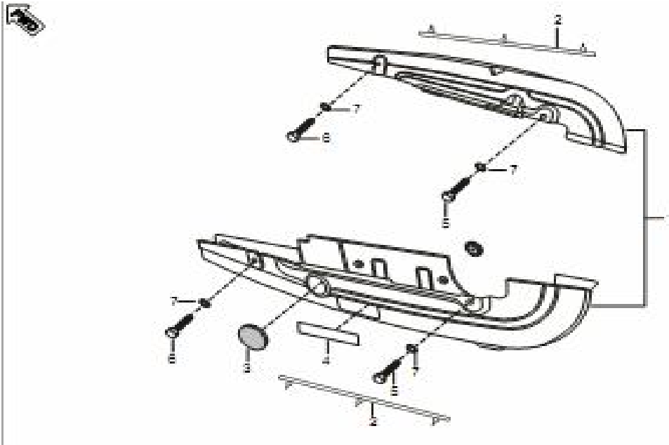
Plate No. 44 : CHAIN CASE
