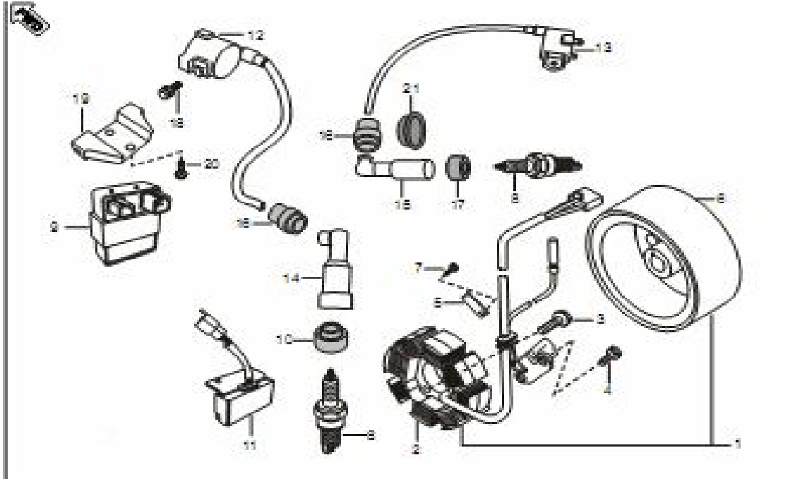
Plate No. 22 : MAGNETO / C.D.I. / H.T. COIL
