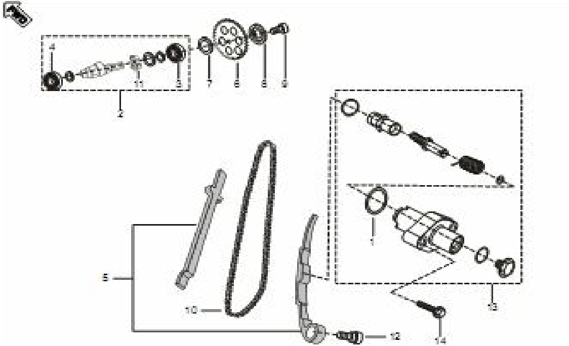
Plate 4:CAMSHAFT/TENSIONER
