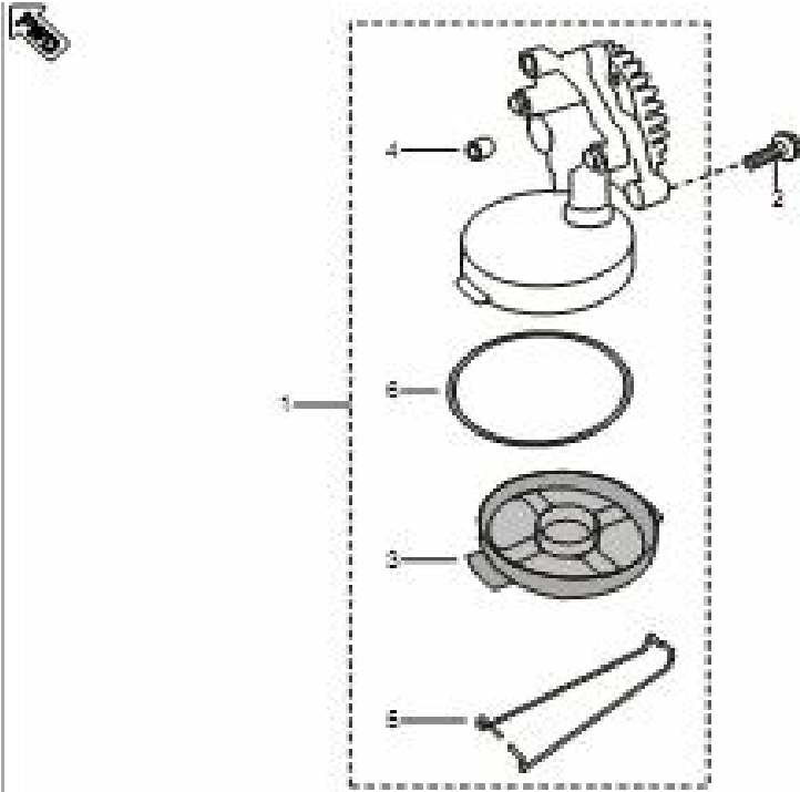
Plate No. 21 : OIL PUMP
