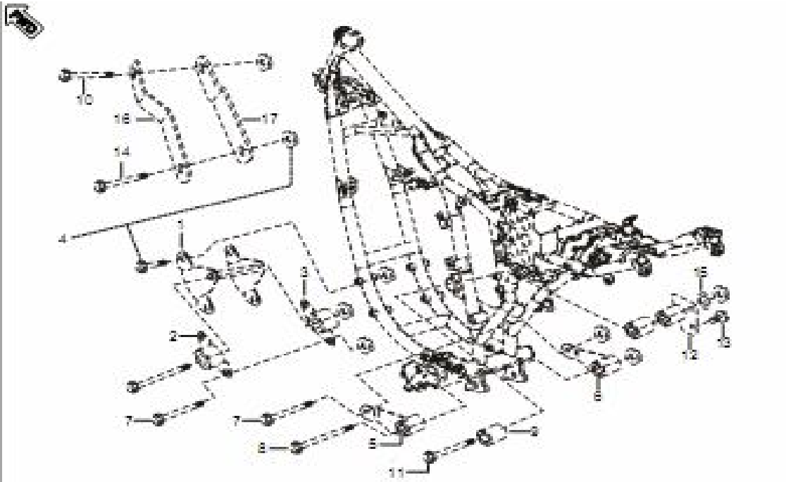
Plate No. 24 : ENGINE MOUNTINGS
