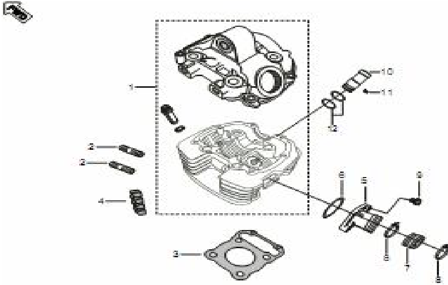
Plate 2: CYLINDERHEAD
