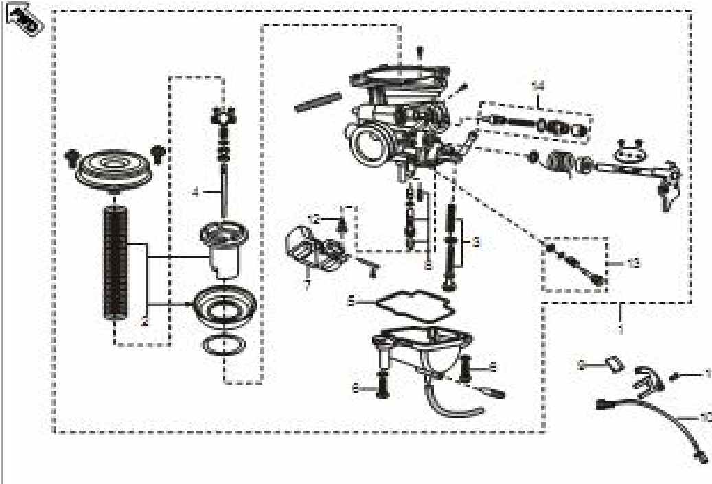
Plate No. 17 : CARBURETTOR
