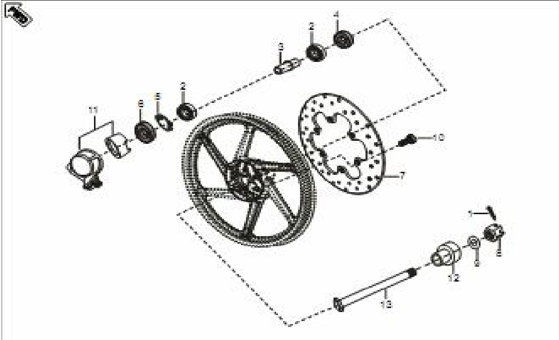
Plate No. 32 : FRONT HUB (FOR DISC BRAKE)
