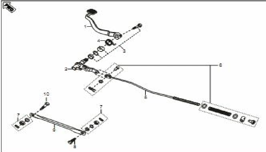
Plate No. 36 : REAR BRAKE PADAL
