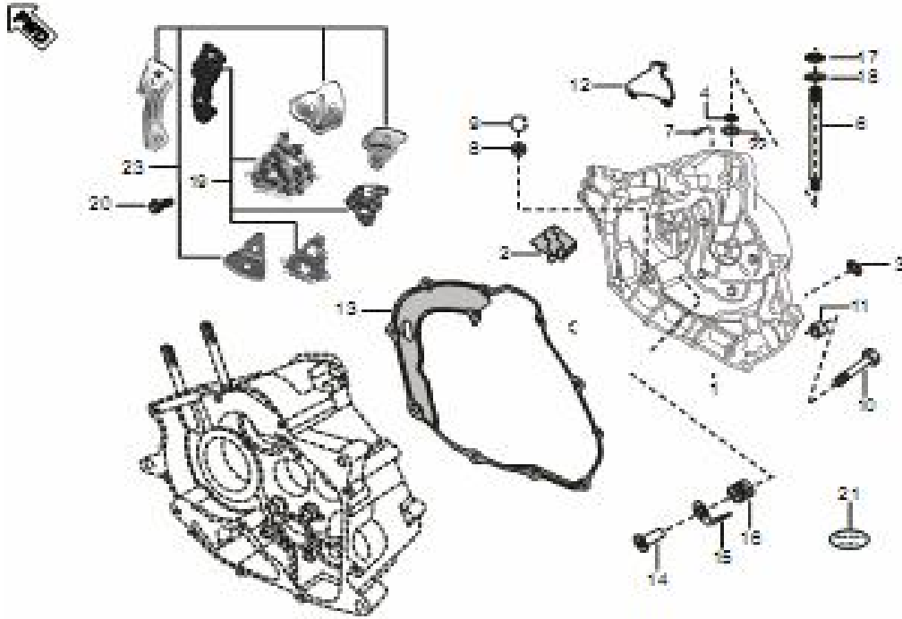
Plate No. 13 : COVER RH
