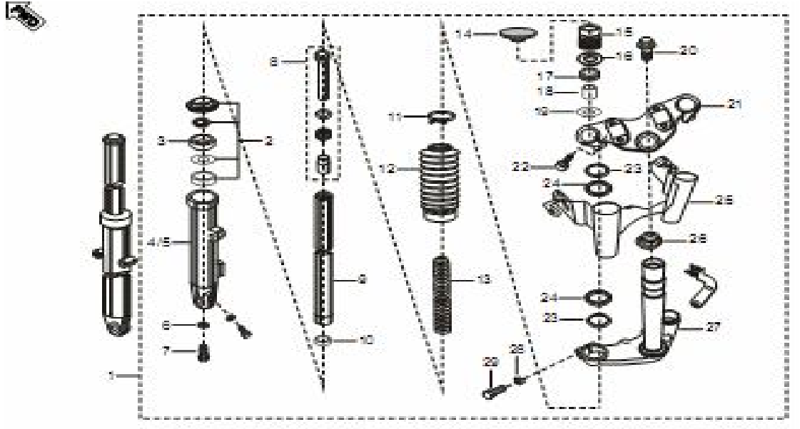
Plate No. 38 : FRONT FORK
