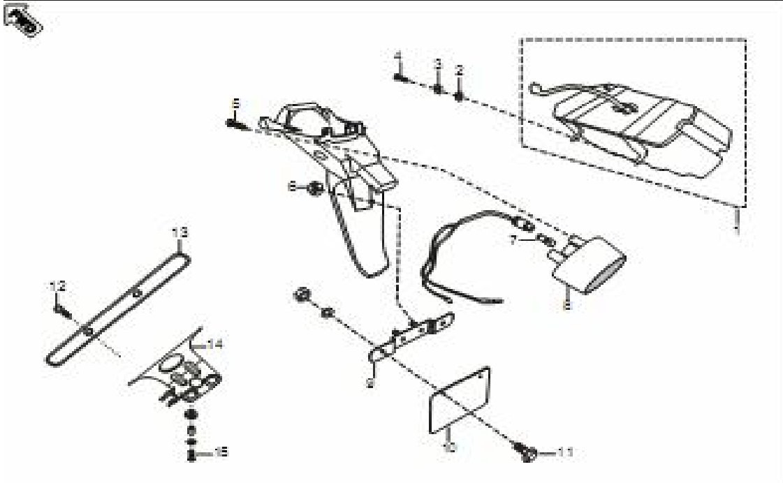
Plate No. 47: TAIL LAMP ASSY & NO PLATE
