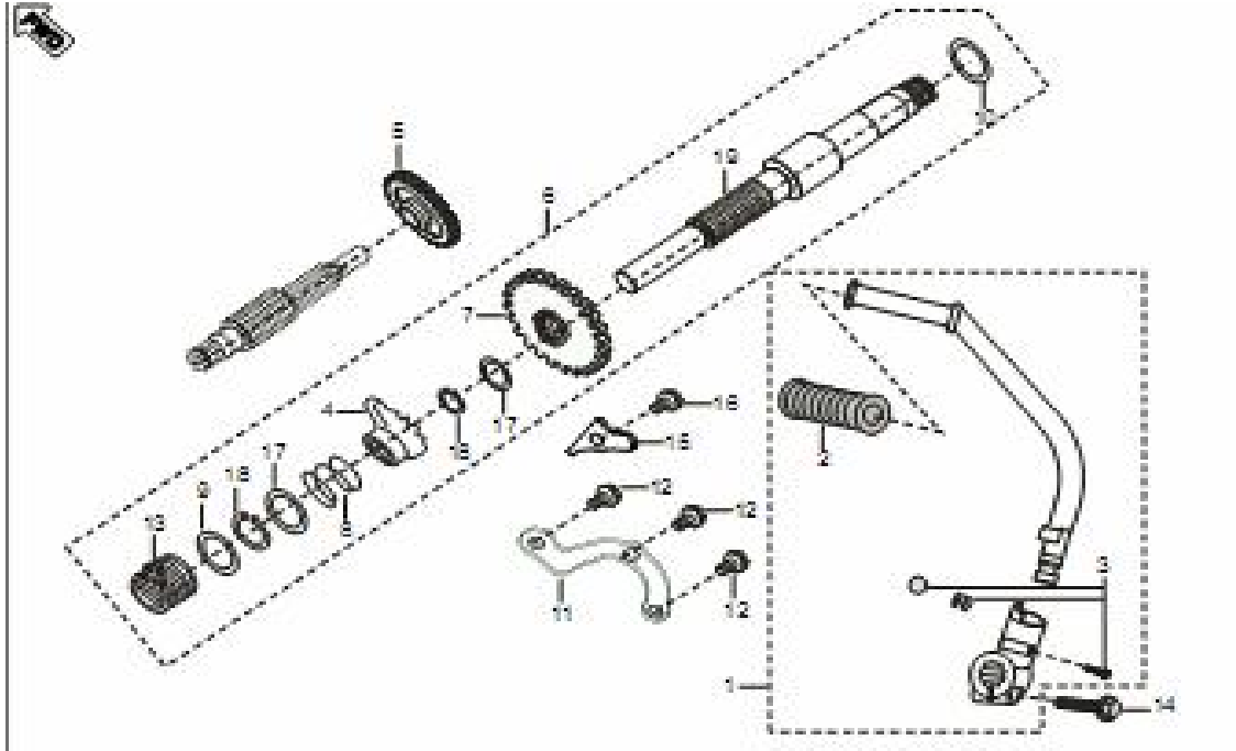
Plate No. 16 : KICK STARTER MECHANISM
