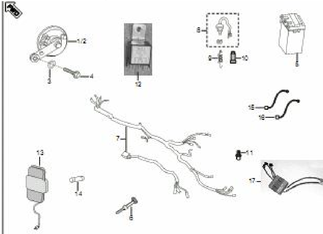
Plate No. 48 : ELECTRICAL EQUIPMENTS
