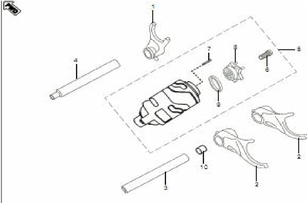
Plate No. 9 : CHANGE DRUM / SHIFT FORK
