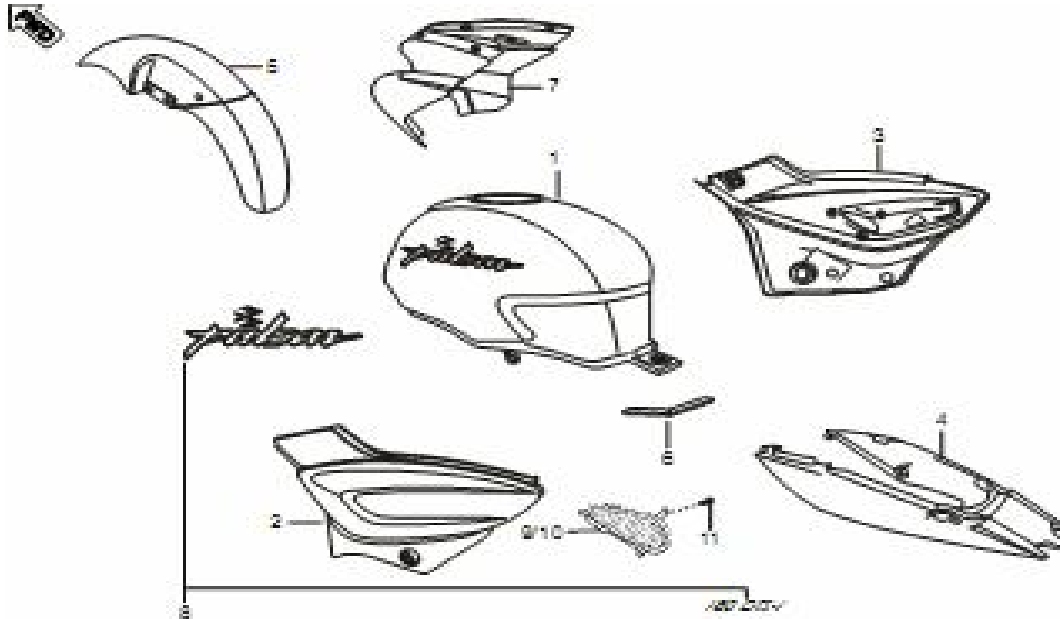
Plate No. 39 : PAINTED PARTS & DECALS
