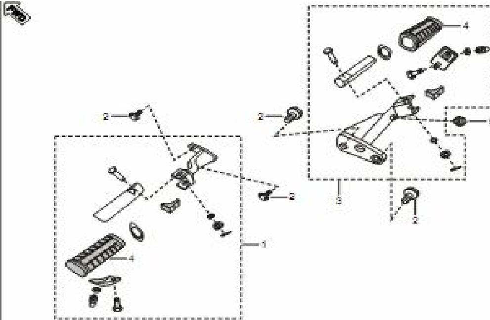
Plate No. 27 : RIDER FOOT REST
