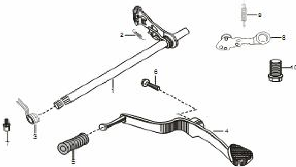
Plate No. 10 : GEAR CHANGE MECHANISM
