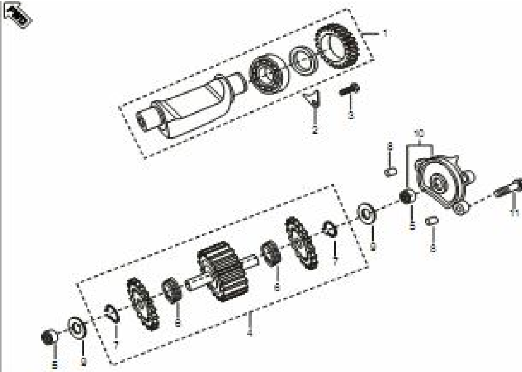
Plate No. 7 : BALANCER & BALANCER IDLER GEAR
