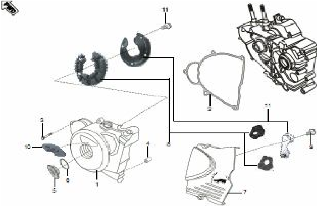
Plate No. 14 : COVER MAGNETO
