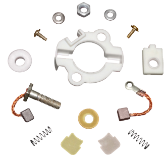
CARBON BRUSH SET W/PLATE UNICORN / SUP. SPL. / CBZ N/M ACU119B
