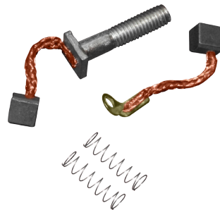
CARBON BRUSH SET W/BOLT UNICORN / SUP. SPL. / CBZ N/M ACU119A
