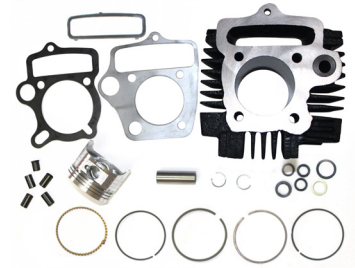
CYLINDER BLOCK KIT (VD) HH VCBK002
