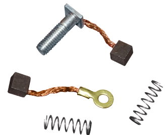
CARBON BRUSH SET (LUCOS TYPE) PULSAR 180 CC VCBS004
