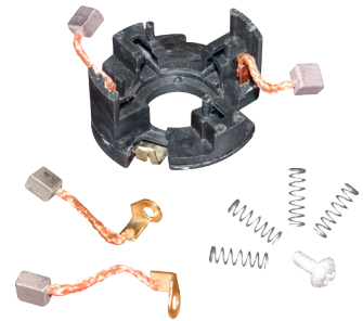
CARBON BRUSH SET W/PLATE APPACHE VCBS012A
