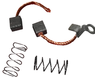
CARBON BRUSH SET N/M SCOOTY VCBS007
