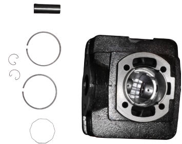
CYLINDER BLOCK KIT SCOOTY VCBK011
