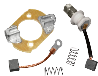
CARBON BRUSH SET (VARAC) W/ Plate PULSAR VCBS013
