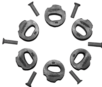
CLUTCH RUBBER KIT (SET OF 12) YAMAHA GF VCRK011
